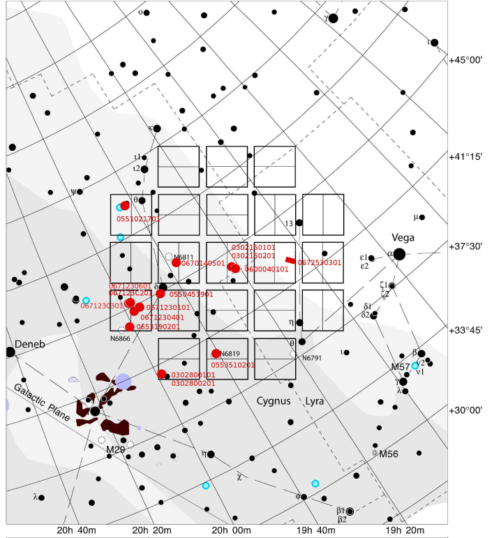
Fig. 1: The field of view (FoV) of the Kepler mission is represented by the solid black squares. It is centered at RA=19 22 40.0, DEC=+44 30 0.0, between the Cygnus and the Lyra constellation. The FoVs of the sixteen 3XMM-DR5 observations we analysed (Table 1) are reported as red circles; the red numbers represent the 3XMM-DR5 unique observation ID (OBS_ID). The FoVs of some XMM-Newton observations are totally or partially overlapping.
