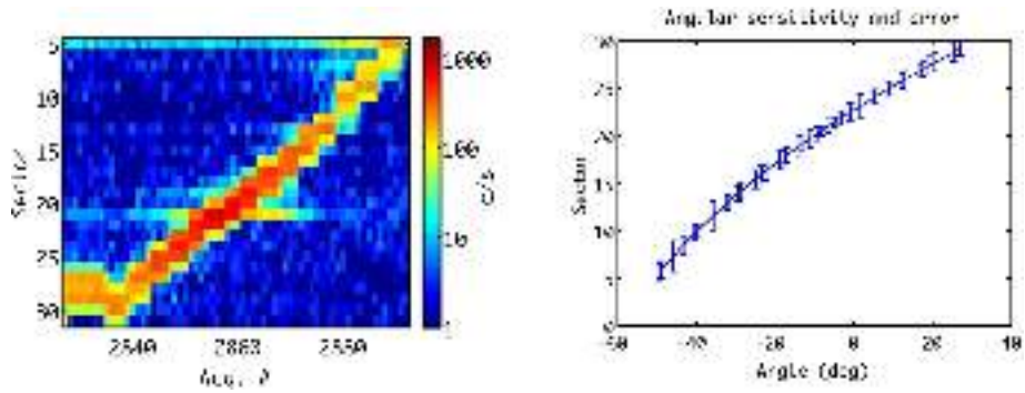
Fig. 47 1-keV O angular scan vs acquisition number ( left ), T_{int}=10 s. The sector distribution of the scanning as a function of incidence angle ( right ) shows the angle-sector correspondence and spread. Note that the efficiency is lower at higher angle as shown by the normalization factor (below)
