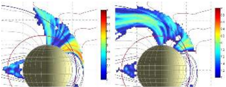
Fig. 8 Colour-coded precipitating (pitch angle < 90°, left panel) and the mirrored (pitch angle > 90°, right panel) proton flux in case of IMF (−20, 0, −5) nT at aphelion. Sample orbit of the MPO spacecraft (red line) and Mio (blue line) with magnetic field-lines are traced in the xz plane (Massetti private communication)
