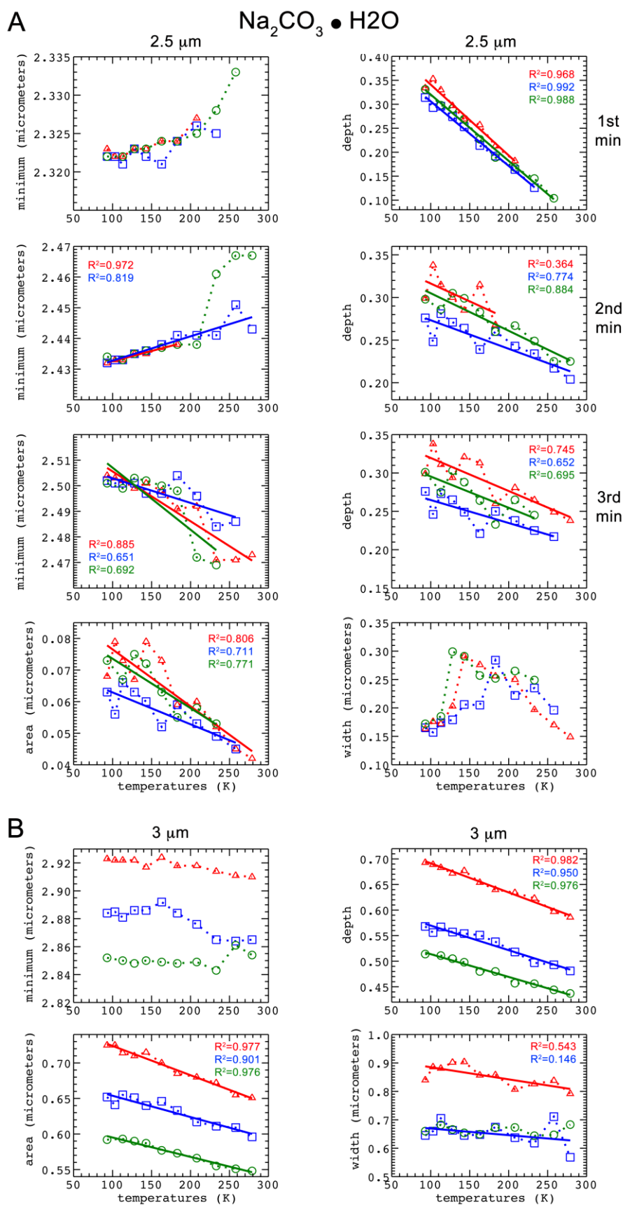
Figure 9. \text{Na}_2\text{CO}_3 \cdot \text{H}_2\text{O} band parameters of 2.32 \mu\text{m} (I), 2.44 \mu\text{m} (II) and 2.50 \mu\text{m} (III) features and 3.0 \mu\text{m} band. Red triangles: 36-50 \mu\text{m} . Blue squares: 75-100 \mu\text{m} . Green circles: 125-150 \mu\text{m} .
