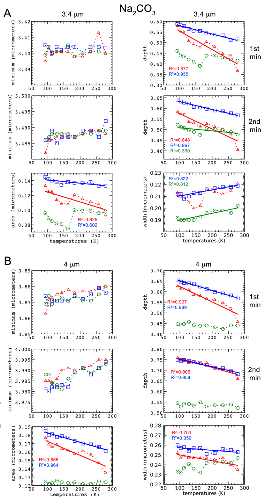
Figure 6. Na 2 CO 3 , band parameters of 3.40 \mu m (I) and 3.49 \mu m (II), and 3.88 \mu m (I) and 3.99 \mu m (II) features. Red triangles: 36-50 \mu m. Blue squares: 75-100 \mu m. Green circles: 125-150 \mu m.
