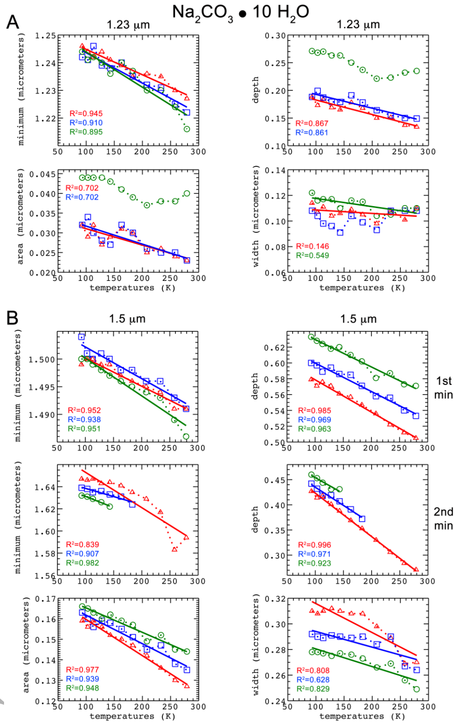
Figure 10. \text{Na}_2\text{CO}_3 \bullet 10\text{H}_2\text{O} band parameters of 1.23\text{-}\mu\text{m} , 1.50\ \mu\text{m} (I) and 1.65\ \mu\text{m} (II) features. Red triangles: 36\text{-}50\ \mu\text{m} . Blue squares: 75\text{-}100\ \mu\text{m} . Green circles: 125\text{-}150\ \mu\text{m} .
