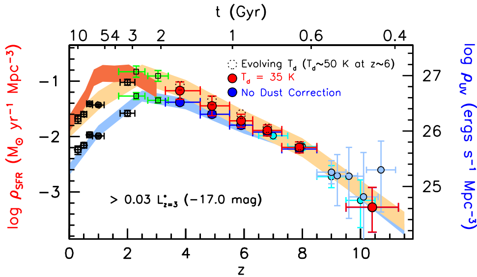
Figure 15. Updated determinations of the derived SFR ( left axis ) and UV luminosity ( right axis ) densities vs. redshift (Section 5.4). The left axis gives the SFR densities we would infer from the measured luminosity densities, assuming the conversion factor of Madau et al. (1998) relevant for star-forming galaxies with ages of \gtrsim 10^8 yr (see also Kennicutt 1998). The right axis gives the UV luminosities we infer by integrating the present and published LFs to a faint-end limit of -17 mag ( 0.03 L_{z=3}^* )—which is the approximate limit we can probe to z \sim 8 in our deepest data set. The upper and lower sets of points ( red and blue circles , respectively) and shaded regions show the SFR and UV luminosity densities corrected and uncorrected for the effects of dust extinction. The dust correction we utilize relies on an IRX– \beta relation intermediate between SMC and Calzetti for the highest-mass galaxies in the present samples, i.e., > 10^{9.75} M_{\odot} , but an IRX–stellar mass relation for lower-mass sources (Section 4.2). The dotted black open circles indicate the dust-corrected SFR densities, assuming an unevolving IRX–stellar mass relation (appropriate if the dust temperature increases monotonically toward high redshift: see Figure 13). The dark red shaded region include the contribution from IR-bright sources (Magnelli et al. 2009, 2011, 2013). Also shown are the SFR densities at z \sim 2-3 from Reddy et al. (2009: green crosses ), at z \sim 0-2 from Schiminovich et al. (2005: black hexagons ), at z \sim 7-9 from McLure et al. (2013) and Ellis et al. (2013: cyan solid circles ), and at z \sim 9-11 from CLASH (Zheng et al. 2012; Coe et al. 2013; Bouwens et al. 2014a: light blue circles ) and Oesch et al. (2013: light blue circles ). The z \sim 9-11 constraints on the UV luminosity density have been adjusted upwards to a limiting magnitude of -17.0 mag assuming a faint-end slope \alpha of -2.0 (consistent with our constraints on \alpha at both z \sim 7 and z \sim 8 ).
