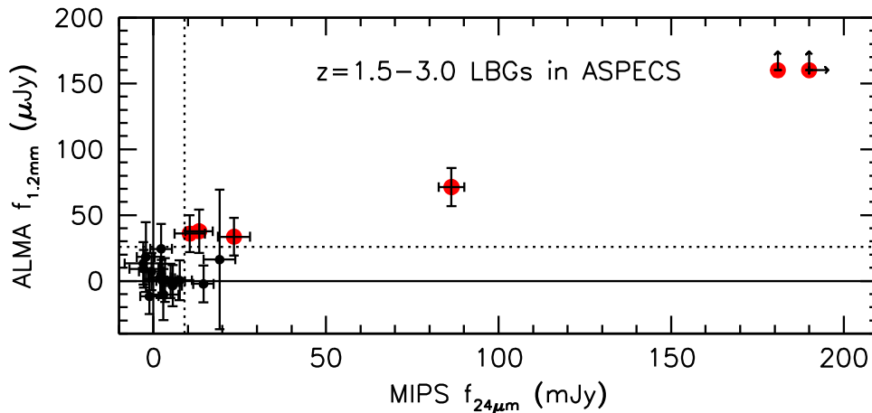
Figure 19. Comparison of the observed MIPS 24\ \mu\text{m} fluxes (Whitaker et al. 2014) for sources in our z \sim 1.5\text{--}3.0 LBG sample with the 1.2\ \text{mm} continuum fluxes measured from ASPECS (solid black circles with 1\sigma error bars shown). The larger solid red circles correspond to the sources for which we claim detections or tentative ALMA 1.2\ \text{mm} detections. The arrows indicate that the measured fluxes lie outside the bounds of the figure. The horizontal and vertical dotted lines show the approximate flux levels where 2\sigma detections are expected. The MIPS 24\ \mu\text{m} fluxes exhibit a broad correlation with the ALMA 1.2\ \text{mm} fluxes for z \sim 1.5\text{--}3.0 galaxies, and those sources that are detected at >2\sigma in the ALMA observations also tend to show significant >2\sigma detections in the MIPS observations (see Table 10).
