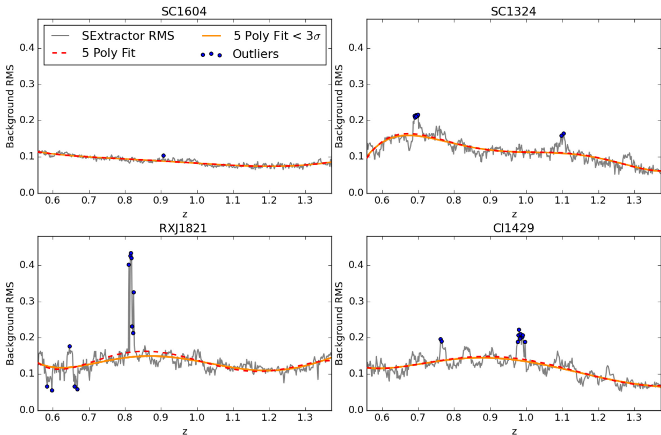
Figure 8. The background RMS as a function of redshift in four fields, SC1604, SC1324, RXJ1821, and CI1429. The grey lines are the background RMS as calculated by SEXTRACTOR. The dashed red line represents a fifth-order polynomial fit without outlier rejection. The solid orange line represents a fifth order polynomial fit with iterative outlier rejection at above 3\sigma , based on the RMS of the preceding polynomial fit. The difference between the two fits with and without outlier rejection is largely minimal outside of areas with large peaks in the background RMS values. SC1604 is a very large field with deep imaging and shows a very flat RMS curve while CI1429 sees a much more variation in its RMS as a function of redshift. SC1324 and RXJ1821 show noticeable peaks at redshifts of 0.7 and 0.8, respectively, which correspond to known large structures in each field.
