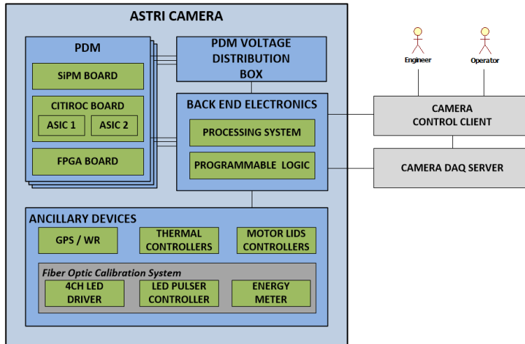
Figure 1. ASTRI SST-2M Camera logical view
