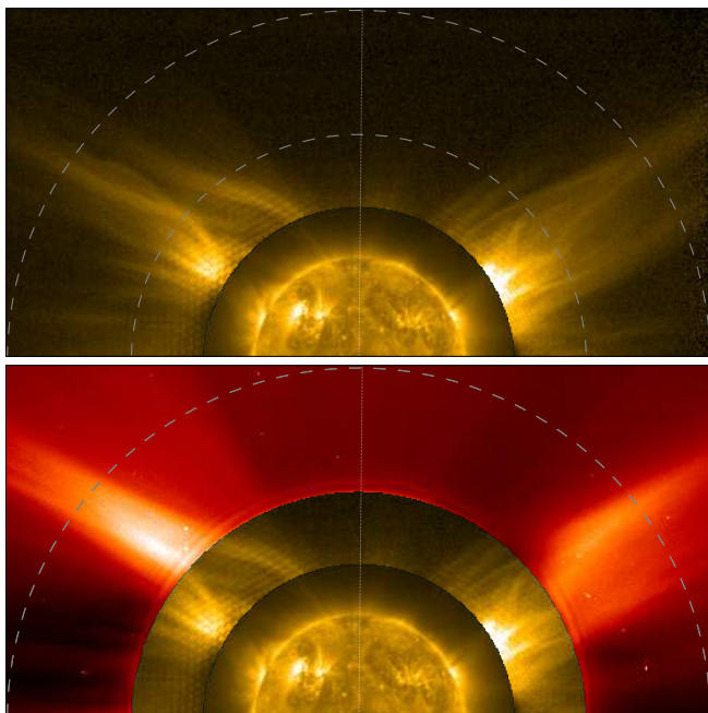
Fig. 11. Comparison of the northern half of the overlapping region between FSI and LASCOCO C2 on 2022 March 7. Top: FSI composite (same images as in Fig. 10), extending to the edges of the detector. The outer dashed circle corresponds to the 3.4 R_{\odot} boundary between FSI and LASCOCO C2 used in Fig. 10. The inner dashed circle corresponds to the boundary between FSI and LASCOCO C2 used in the bottom panel. Bottom: same as above, with LASCOCO C2 above 2.2 R_{\odot} , the inner limit of the useful LASCOCO C2 FOV.
