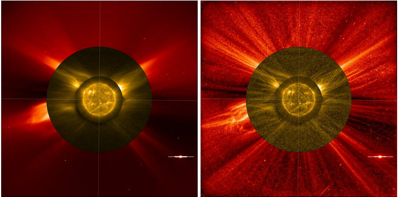
Fig. 10. Composites of images at 17.4 nm from FSI in disk mode (below 1.5 R_{\odot} , 11:29 UT) and coronagraph mode (below 3.4 R_{\odot} , 2022 March 7 16:00 UT) and in VL from LASCOCO C2 (16:12 UT). Left: original LASCOCO C2 and FSI images, displayed using linear and square root scaling, respectively. Right: images enhanced with the WOW filter.
