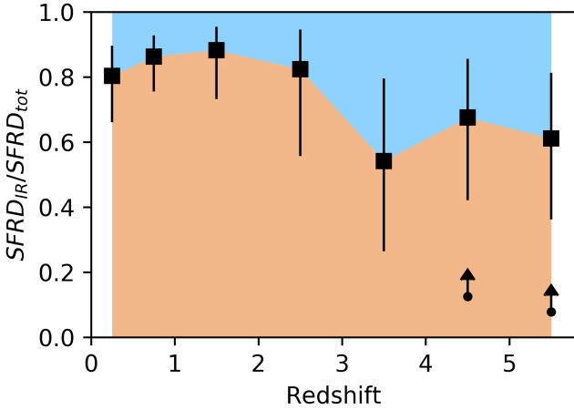
Fig. 9. Evolution of the fraction of the dust obscured \text{SFRD}_{\text{IR}} as a function of redshift. The arrows show the lower limits obtained using the lower limits discussed in Sect. 4.3.1. The points at z < 4 are obtained using a compilation of the literature from Fig. 7. The points at z > 4 are obtained using the UVLF+GSMF combined measurements from Table 2.
