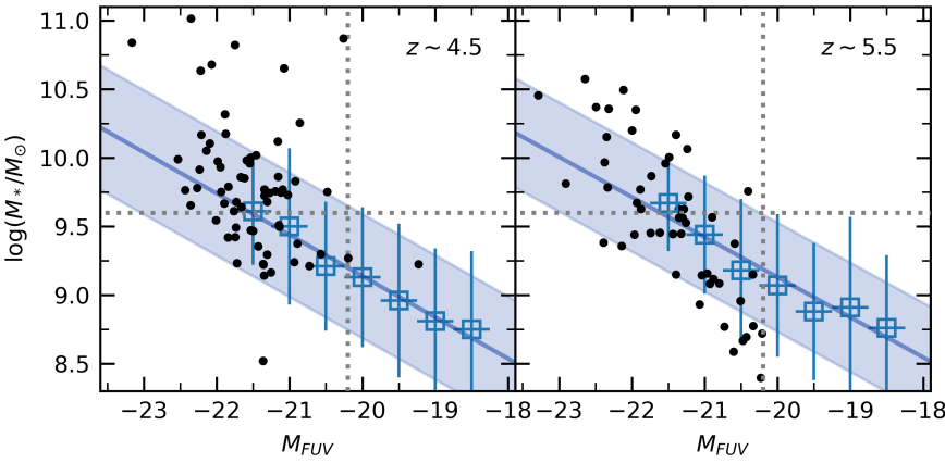
Fig. 3. Stellar mass versus FUV magnitude. The black circles are ALPINE targets as measured by Faist et al. (2020). The open squares are measurements from Salmon et al. (2015). The solid blue line is the fit to the measurements by Salmon et al. (2015) and the shaded areas are 1\sigma uncertainties. The vertical dotted line shows the FUV luminosity cut used in selecting galaxies. The vertical dotted lines show the mass limits below which the flux measurements are considered to be upper limits. Left panel: z \sim 4.5 redshift bin and right panel: z \sim 5.5 bin.
