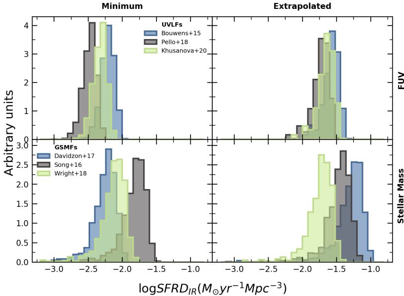
Fig. 6. Same as Fig. 5, but at redshift z \sim 5.5 . The UVLFs and GSMF are taken from Bouwens et al. (2015b), Pello et al. (2018), Khusanova et al. (2020), Davidzon et al. (2017), Song et al. (2016), Wright et al. (2018).
