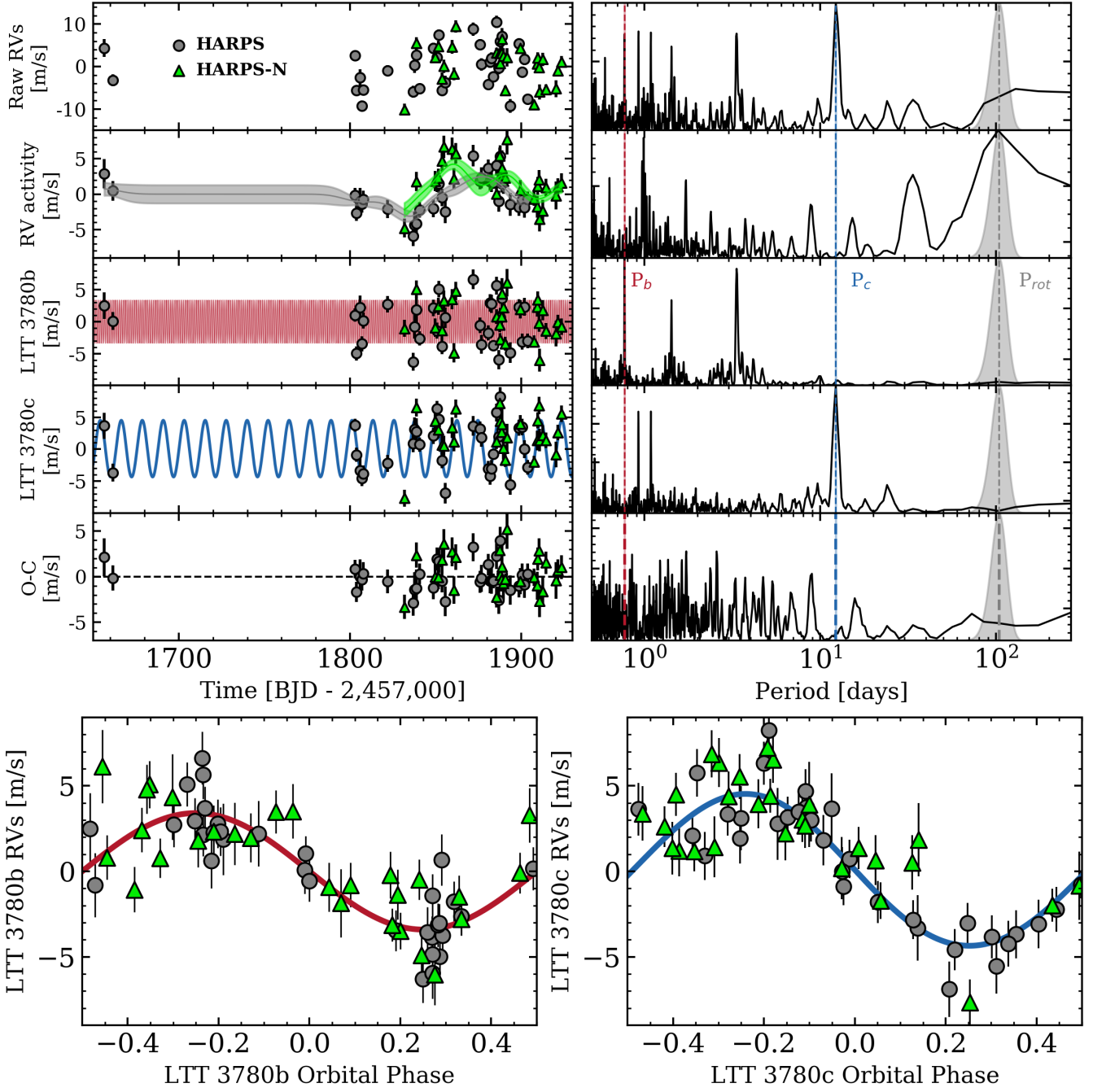
Figure 5. The RV data and individual model components from our analysis of the HARPS ( gray circles ) and HARPS-N ( green triangles ) RV measurements. The data and models are depicted in the left column of the first five rows while their corresponding Bayesian generalized Lomb-Scargle periodograms are depicted in the right column. The marginalized posteriors of the LTT 3780b and c orbital periods are depicted as vertical lines along with the estimated stellar rotation period using the M dwarf activity-rotation relation from Astudillo-Defru et al. (2017) ( P_{rot} = 104 \pm 15 days). First row: the raw RV measurements. Second row: the RV activity signal modeled with a quasi-periodic GP for each spectrograph. Third row: the RV signal from LTT 3780b at 0.77 days. Fourth row: the RV signal from LTT 3780c at 12.25 days. Fifth row: the RV residuals. Bottom row: the phase-folded RV signals of LTT 3780b and c.
