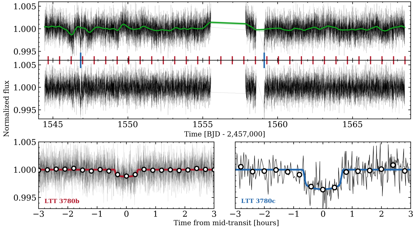
Figure 4. Upper panel: the TESS PDCSAP light curve of LTT 3780 (black curve) along with the mean GP detrending model (green curve) and its 3\sigma confidence interval in the surrounding shaded region which is narrow and hence difficult to discern. The vertical red and blue ticks along the x-axis highlight the mid-transit times of the planets LTT 3780b and c respectively. Middle panel: the detrended TESS light curve. Lower panels: phase-folded light curves of LTT 3780b (left) and c (right) along with their best-fit transit models. White markers depict the temporally-binned phase-folded light curves to help visualize the transit events.
