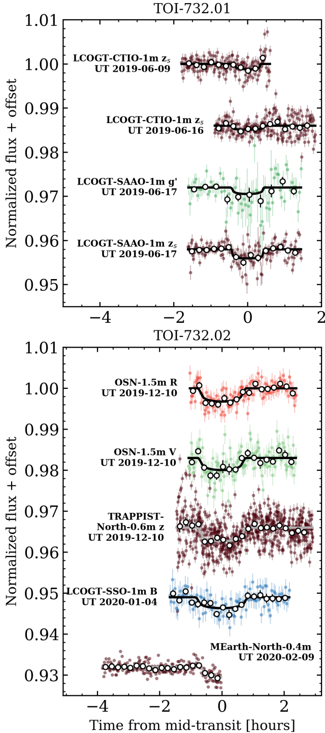
Figure 2. Ground-based transit light curves of TOI-732.01 ( upper panel ) and 02 ( lower panel ) taken as part of TFOP. Solid curves depict the optimized transit model fit with all model parameters fixed other than the baseline flux, the mid-transit time, and the planet-to-star radius ratio. Annotated next to each light curve is the telescope facility, the passband, and the UT observation date.
