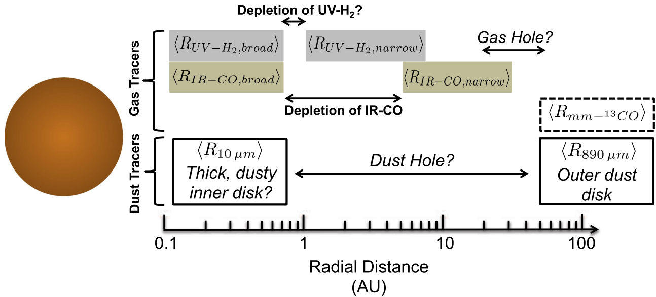
Figure 9. Summary of radial structure in the molecular gas disk, showing average distances for UV-H 2 ( \langle r_{\text{broad,H}_2} \rangle = 0.4 \pm 0.1 au; \langle r_{\text{narrow,H}_2} \rangle = 3 \pm 2 au) and IR-CO ( \langle r_{\text{broad,CO}} \rangle = 0.4 \pm 0.1 au; \langle r_{\text{narrow,CO}} \rangle = 15 \pm 1 au) emission. The mm- 13 CO and 890 \mu\text{m} dust cavities ( r_{\text{cavity}} \sim 50 au) were first observed by Ansdell et al. (2016b) and were modeled by van der Marel et al. (2018). We also consider the location of dust grains producing the 10 \mu\text{m} silicate emission feature, which we interpret as evidence for an optically thick inner dust disk. Taken together, these metrics point to the presence of a gas hole in the inner disk, embedded within a larger dust gap extending from \sim 1 to 50 au.
