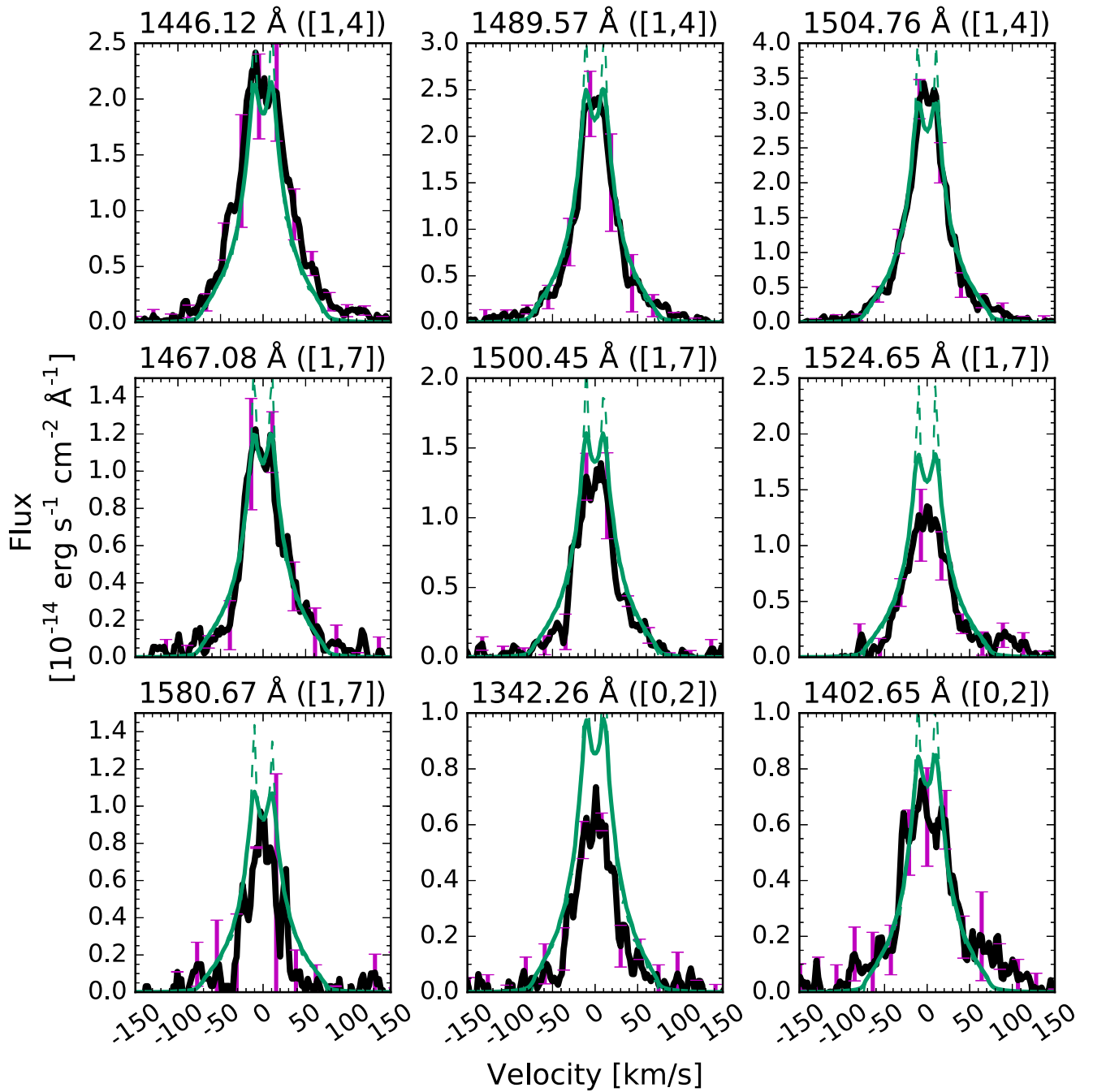
Figure 4. Model line profiles (green) of H 2 fluorescent emission lines from the [1, 4], [1, 7], and [0, 2] progressions (black), produced with the median values from the posterior distributions of the parameters. All nine lines were fit simultaneously, and the corresponding model parameters inform us about the radial structure of the emitting gas. The dashed green lines show the model line profiles before they were convolved with the HST -COS line-spread function.
