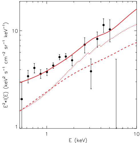
Figure 5. The spectrum of the uCXB ( circles ) as measured with Chandra ACIS-I in this work. The uCXB spectrum is compared with AGN synthesis models by Treister et al. (2009) ( red dotted line ), Gilli et al. (2007) ( red continuous line ) and Ballantyne et al. (2011) ( red dashed line ) after the survey X-ray selection function is applied (galactic N_H correction is irrelevant).
