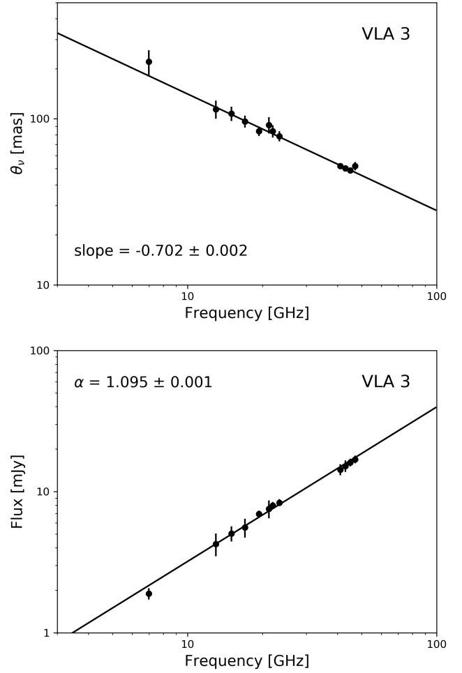
Figure 6. Dependence of the angular size of the jet with frequency (top panel) and spectral energy distribution (bottom panel) of VLA 3. Flux densities and semi-major axes \theta_\nu , are obtained from Gaussian fits to the brightness profile of VLA 3, in 2 GHz bandwidth images. To measure flux densities we use uniform-weighted images (C band) and natural-weighted images (Ku, K, and Q bands), while angular sizes were measured in uniform-weighted images (C, Ku, and K bands) and Briggs-weighted (robust -1) images (Q band). Solid lines are linear least-squares fits to the log data. Angular size error bars correspond to fitting errors, while flux error bars consider both fitting and calibration errors.
