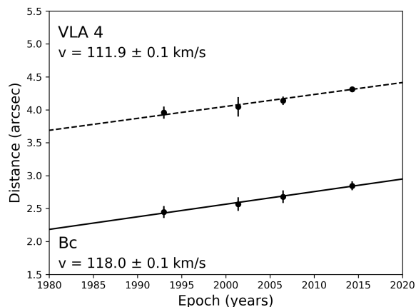
Figure 7. Proper motion diagrams for the Bc and VLA 4 sources. Positions are computed as the distances to the averaged coordinates of the system VLA 1–VLA 2–VLA 3 in four epochs (1992.98, 2001.40, 2006.47, 2014.29): RA(J2000) = 20h 38m 36.47s, DEC(J2000) = 42° 37′ 34.15″. The solid lines are least-square fits to the data. Velocities on the plane of sky are derived by assuming a distance to the region of 1.3 kpc (Rygl et al. 2012). Bc and VLA 4 are moving away from the system with PAs of \sim 20^\circ and \sim 10^\circ , respectively.
