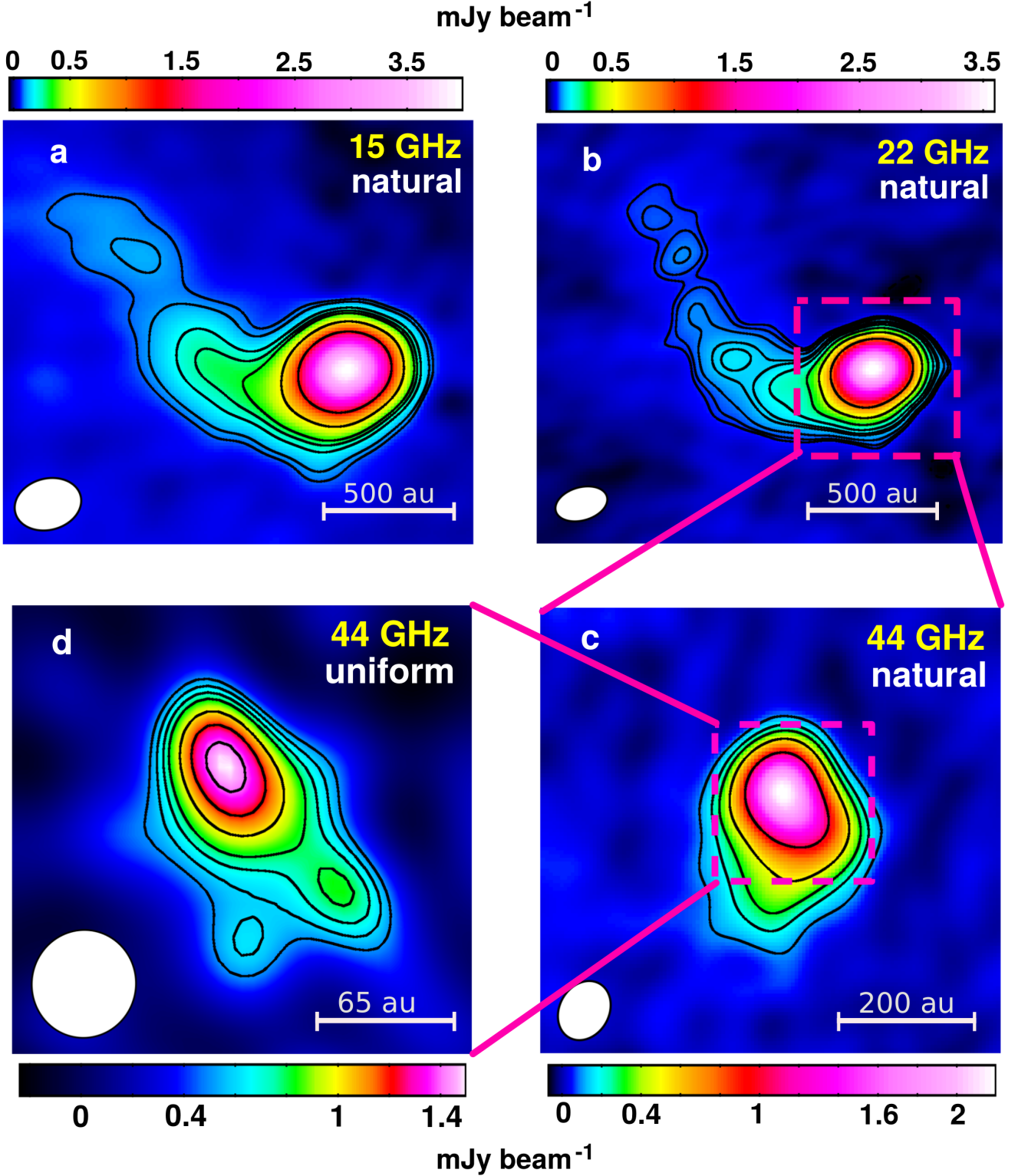
Figure 4. VLA 1 continuum emission (epoch 2014.29). (a) Natural-weighted image at Ku band (central frequency 15 GHz); contours are -3, 6, 8, 15, 20, 25, 50, and 100 \times 10 \mu\text{Jy/beam} , the rms of the map. The synthesized beam is 0''.21 \times 0''.16 , PA = -75^\circ . (b) Natural-weighted image at K band (central frequency 22 GHz); contours are -3, 6, 7, 9, 13, 15, 20, 30, 50, 100 \times the rms = 10 \mu\text{Jy/beam} . The synthesized beam is 0''.16 \times 0''.10 , PA = -74^\circ . The magenta dotted rectangle indicates the zoomed-in region shown in panel (c). (c) Natural-weighted image at Q band (central frequency 44 GHz); contours are -3, 5, 10, 15, 25, 50 \times the rms = 20 \mu\text{Jy/beam} . The synthesized beam is 0''.07 \times 0''.05 , PA = -29^\circ . The magenta dotted rectangle indicates the zoomed-in region shown in panel (d). (d) Uniform-weighted image at Q band; contours are -3, 5, 6, 7, 8, 10, 12, 14 \times the rms = 100 \mu\text{Jy/beam} . The synthesized beam is 0''.038 \times 0''.037 , PA = -9^\circ . The physical scale of 65 au corresponds to 0.05 arcsec.
