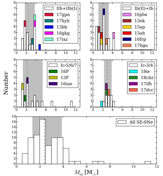
Figure 15. The M_{\text{ej}} distribution of SNe I Ib + I Ib(I) (top left), SNe Ib(II) and Ib (top right), SNe Ic-5/6/7 (middle left), and SNe Ic-3/4 (middle right), and all SE-SNe including GRB and XRF-SNe (lower panel). The dashed line and grey regions are as in Fig. 9.
