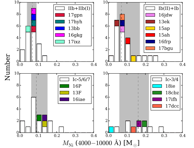
Figure 14. The distribution of M_{Ni} synthesized through explosive Si burning after core-collapse and calculated using the 4000–10 000 Å light curve. Only SNe where E(B - V)_{host} is known are included. The dashed line and grey regions are as in Fig. 9. SNe Ibc have not been classified conclusively as either SNe Ic or SNe Ib.
