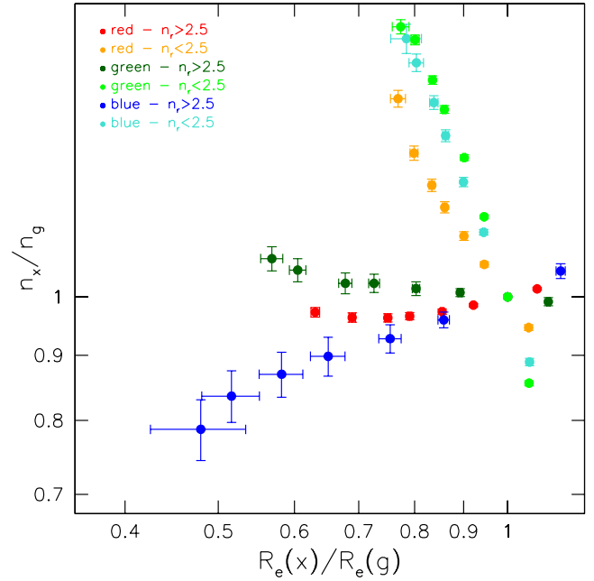
Figure 17. Median \mathcal{N}_g^x versus median \mathcal{R}_g^x for galaxies in each of our different subsamples divided by colour and Sérsic index. Symbols are as usual. Multiple points of the same symbol correspond to different wavebands, x . These consistently follow the wavelength sequence from H on the left to u on the right. All the g -band points lie at (1, 1) by definition.
