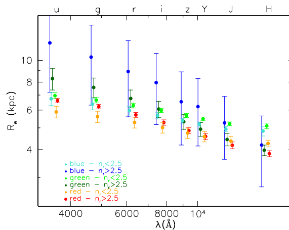
Figure 13. Median effective radius as a function of wavelength for galaxies of different colour and Sérsic index. Red, dark green and blue symbols represent high- n galaxies; orange, light green and turquoise symbols low- n galaxies. Error bars represent the uncertainty on the median. The median effective radius depends on wavelength. Small offsets in wavelength have been applied to all points for clarity. Low- n samples display similar behaviour, while the high- n samples show stronger, and more varied, trends.
