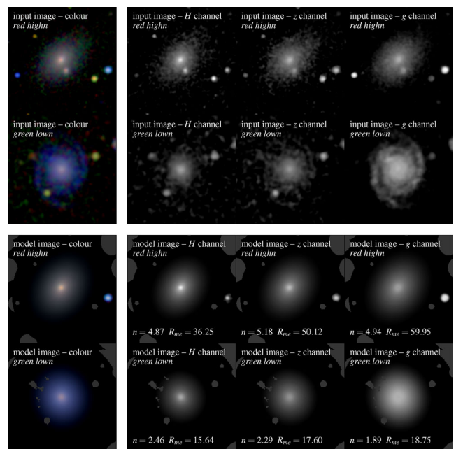
Figure 19. Left: example Hzg images of a red, high- n and a green, low- n galaxy, each with typical dependences of n and R_e on wavelength (they lie at the peaks of their respective distributions in Fig. 18). The images are displayed using the colour-preserving method of Lupton et al. (2004), with an asinh stretch to reveal the full range of surface brightness. The upper panels show the data, while the lower panels show the GALFITM model. Grey regions in the model images indicate where pixels were masked during the fit. Right: individual red, green and blue bands from the colour images, which make it easier to appreciate the relative distributions of the H -, z - and g -band light. For both galaxies, the central region is significantly redder than the outskirts. This is more subtle for the high- n galaxy, as n is stable with wavelength, but still amounts to an increase in R_e by almost a factor of 2 between the H and g bands.
