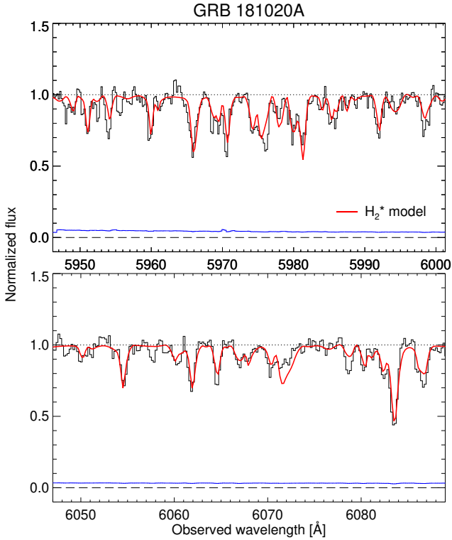
Fig. 3. Normalized VLT/X-shooter VIS arm spectrum of GRB 181020A showing regions encompassing a subset of the strongest H_2^* lines. The solid black lines show the data, the blue lines the associated error and the red lines the best-fit model.
