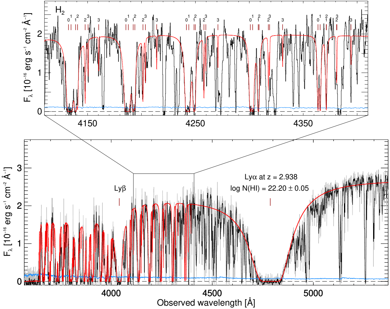
Fig. 1. VLT/X-shooter UVB arm spectrum of GRB 181020A. The absorption features from the H I Ly\alpha , Ly\beta and H_2 Lyman-Werner band line transitions are clearly shown. The raw spectrum is shown in gray with the associated error spectrum in blue. A binned version of the spectrum is overplotted in black. A synthetic spectrum of the best fit model to H I and H_2 is shown as the solid red line and the Ly\alpha and Ly\beta absorption features are marked at the observed redshift of z = 2.938 . Top panel: a zoom-in of a subset of the most constraining Lyman-Werner band line transitions from molecular hydrogen. The redshifted wavelengths of the strongest rotational levels J = 0, 1, 2, 3 are marked above each line.
