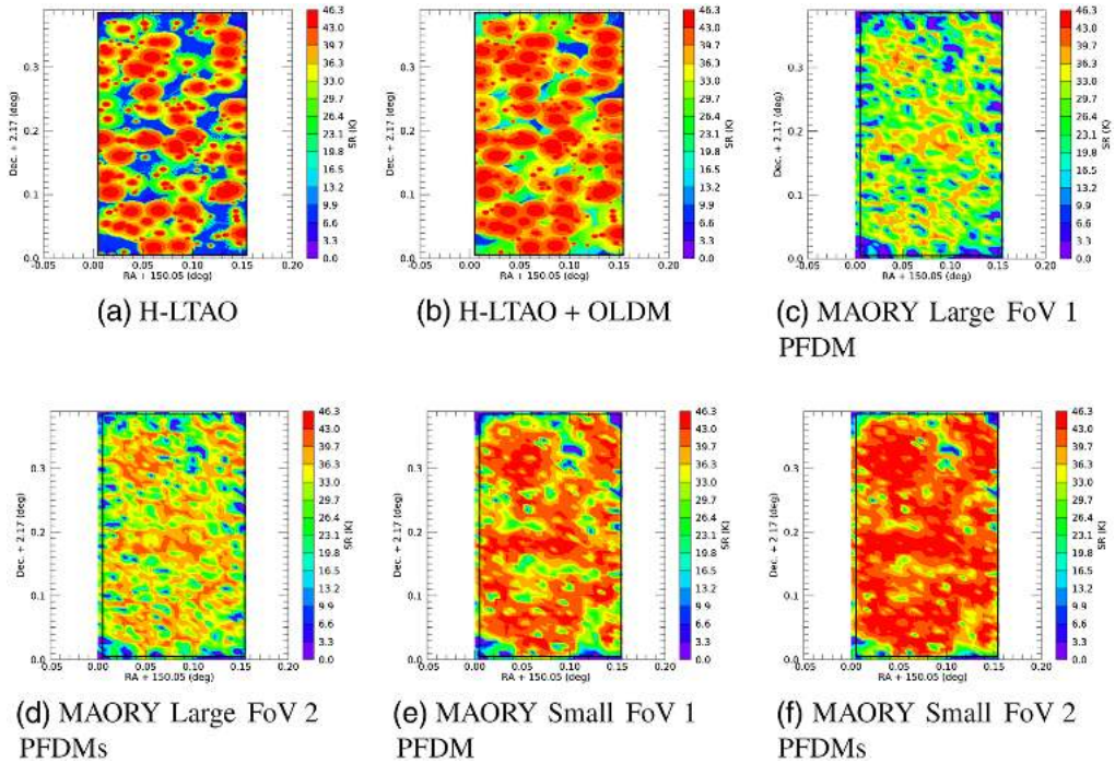
Fig. 10 SNR in K band with H-LTAO (on axis) or with MAORY (averaged on the scientific FoV) for the COSMOS field. The black lines indicate the area used for the SC computation.
