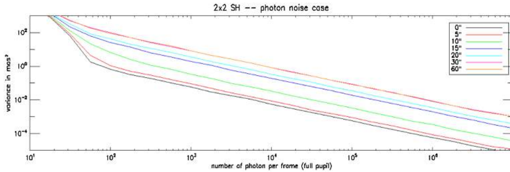
Fig. 4 Example of noise computed for a 2 × 2 SHWFS, for different level of fluxes, and different position of the NGS in the field, in the case of an LTAO correction without OLDLM.
