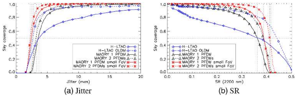
Fig. 7 SC with H-LTAO or with MAORY at l = 90 deg, b = -60 deg. The jitter/SR is on axis for H-LTAO and averaged on a 1 arcmin diameter FoV (large FoV) or on a 20'' diameter FoV (small FoV) for MAORY.
