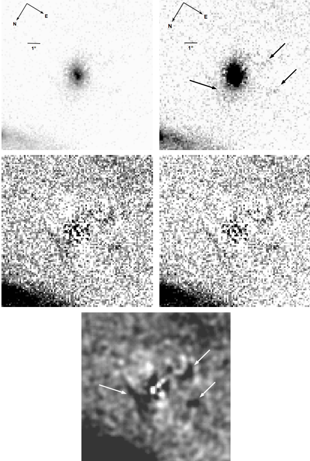
Figure 3. View of the AGN host galaxy and residuals. The field of view is the same as in Fig. 1. Top row: The PSF and Galaxy B models have been subtracted, showing the AGN host galaxy. Top left: Low-contrast image, showing the inner features of the host. The noise 1 arcsec from the host centre is due to scaling up the faint edges of the stellar PSF model. Top right: High-contrast image, emphasizing the outer envelope. Three clumps of material are indicated by the arrows. The lower two are just visible in Fig. 1 but are clearer here. The clump to the southeast of the AGN is hidden by Galaxy B in the original image. Middle row: Residuals made by subtracting the total model. An inverted color scheme (blackier is brighter) is used, in keeping with the images at top. Middle left: 1C model residual. Middle right: 2C model residual. The higher noise at the centre, extending to a radius of 1 arcsec, is due to the PSF model. The apparent structures noted in the top row stand out above the variations in the sky and residual. Bottom: 1C model residual with 3-pixel Gaussian smoothing. The clumps of material noted before (marked with arrows) are more visible.
