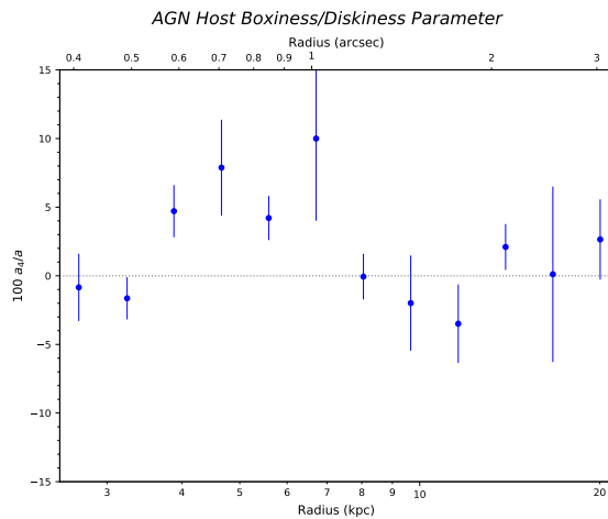
Figure 6. Isophote boxiness/diskiness parameter as a function of semi-major axis. Negative values of a_4 < 0 indicate boxiness, while positive values indicate diskiness. Using the criteria of Bender et al. (1989), we can assign a characteristic value of a_4/a \sim 0.05 - 0.08 , which is discy.
