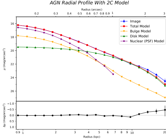
Figure 5. Radial surface brightness ( \mu ) plot of the AGN image and components for the 2C (Sérsic bulge + exponential disc) model. The plot layout and scale are the same as in Fig. 4. The Sérsic + exponential disc model is a good match to the profile out to about 1.8 arcsec (12 kpc). From there to about 3 arcsec (20 kpc), there is excess light from the filament-like structure to the north and imperfectly-subtracted light in Galaxy B, both shown in the residual image in Fig. 3. Though the 2C model’s radial profile diverges from the image in the outer radii, it provides a better overall fit in two dimensions than the 1C model does.
