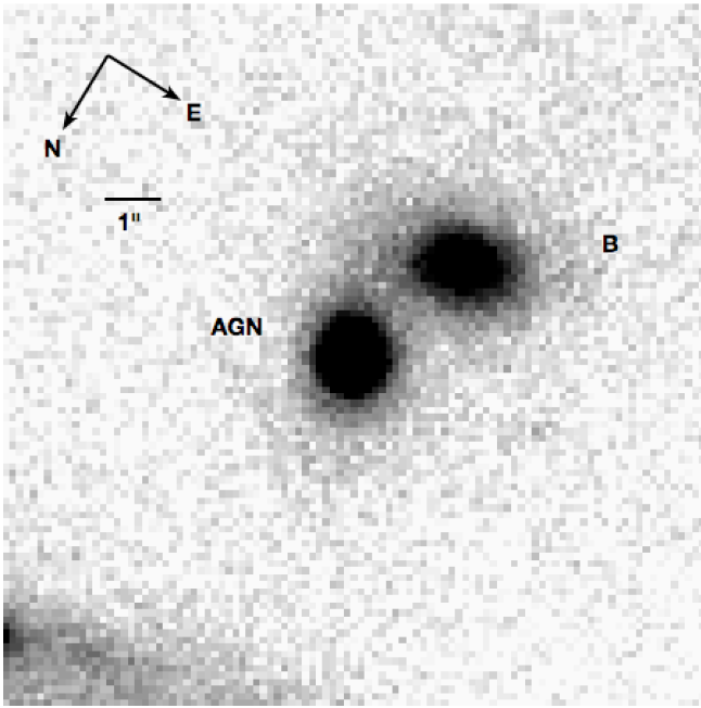
Figure 1. J -band view of the field surrounding SBS 0846 + 513. SBS 0846 + 513 is marked ‘AGN,’ and the projected companion ‘B.’ At bottom, an arm from a large, foreground spiral can be seen. The scale bar spans 1 arcsec.
