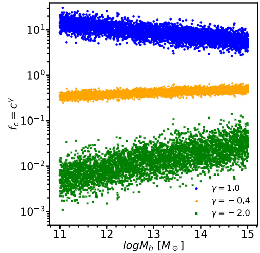
Figure 4. Scatter induced by different choices of \gamma in the factor f(c) = c^\gamma as a function of halo mass. Blue dots, orange triangles and green crosses are for \gamma = 1 , -0.4 , and -2.0 , respectively. Concentrations are from Dutton & Macciò (2014).
