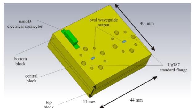
Figure 3: 3D view of the bottom part of the OMT receiver module showing the orientation of the two oval output waveguides. The external dimension of the assembled blocks is 40 x 44 x 13 \text{mm}^3 .
