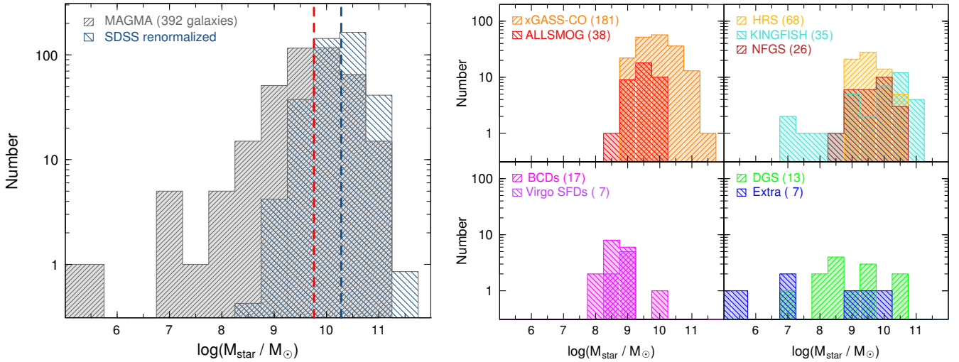
Fig. 2. Distributions of M_{\text{star}} for the MAGMA sample; the right panels illustrate the subdivisions in M_{\text{star}} for the parent surveys. The red vertical dashed line in the left panel corresponds to the median M_{\text{star}} for MAGMA, \log(M_{\text{star}}/M_{\odot}) = 9.68 . Also shown in the left panel is the SDSS10 sample, taken from Mannucci et al. (2010), consisting of 78579 galaxies. Here, it has been renormalized to show the M_{\text{star}} distribution it would have if it contained the same number of galaxies (390) as MAGMA; the M_{\text{star}} median of SDSS10 (shown as a blue vertical dashed line) is \log(M_{\text{star}}/M_{\odot}) = 10.28 .
