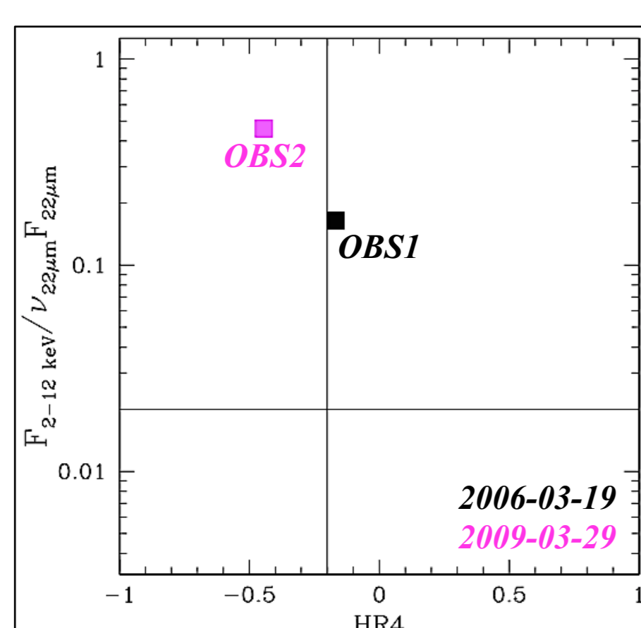
Figure 4. The HR vs. F_X/F_{IR} diagnostic diagram showing the position of the two observations of NGC 6860.
