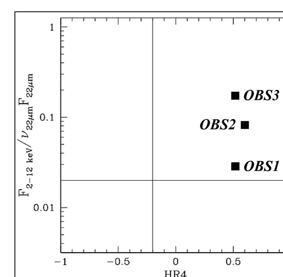
Figure 6. The HR vs. F_X/F_{IR} diagnostic diagram showing the position of the three observations of NGC 4388.
