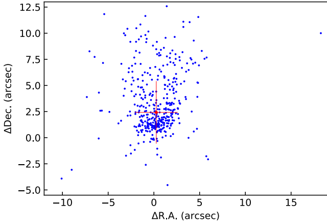
Fig. 2. Differences in the source positions between our observations and the FIRST catalogue. The red cross shows the mean \Delta R.A. and \Delta Dec. of the scatter, where the uncertainties are the standard deviation.
