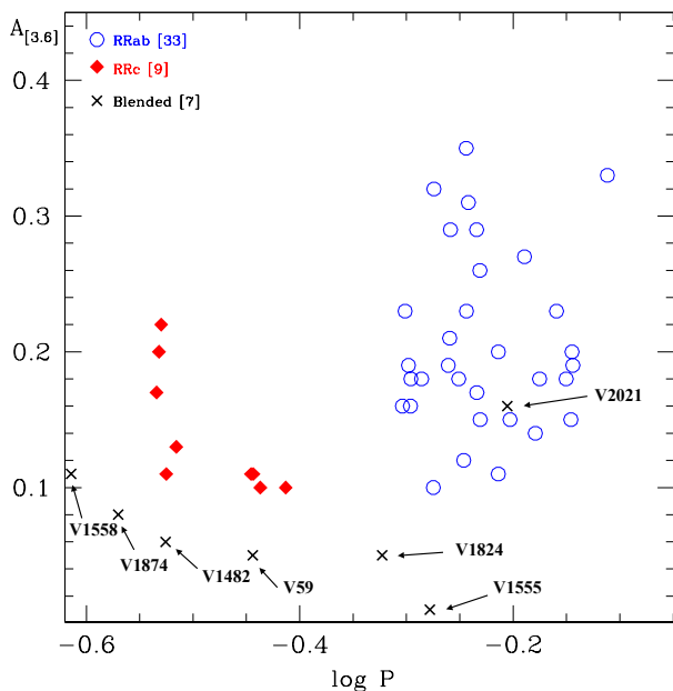
Figure 3. Mid-infrared period-amplitude diagram for all the RRL in our sample based on light curves at 3.6 \mu\text{m} . The blue open circles and the red diamonds mark the RRab and RRc stars respectively. The RRL affected by crowding/blending and discarded in this study are labelled and marked with crosses.
