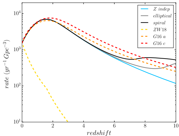
Figure 14. The predicted evolution of SGRB rate against the observed ones. The models shown are the 4A (in light blue) and the 4AV2 (black and grey lines). In particular, the grey line refers to the sub-model with a [\text{Fe}/\text{H}] evolution as predicted for an elliptical galaxy, whereas the black line refers to the sub-model with a [\text{Fe}/\text{H}] evolution as predicted for the Milky Way.
