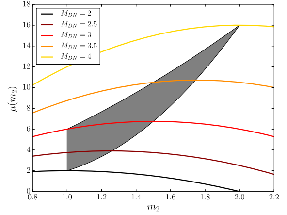
Figure 1. The function \mu(M_{\text{DN}}, m_2) is plotted with respect to m_2 for five different fixed values of M_{\text{DN}} ( 2.0 M_{\odot} in black, 2.5 M_{\odot} in dark red, 3.0 M_{\odot} in red, 3.5 M_{\odot} in orange, and 4.0 M_{\odot} in yellow solid lines). The grey shaded area represents the space of valid values for m_2 (i.e. represents a system with a secondary lighter than the primary and in the correct mass range, for a fixed total mass of the system).
