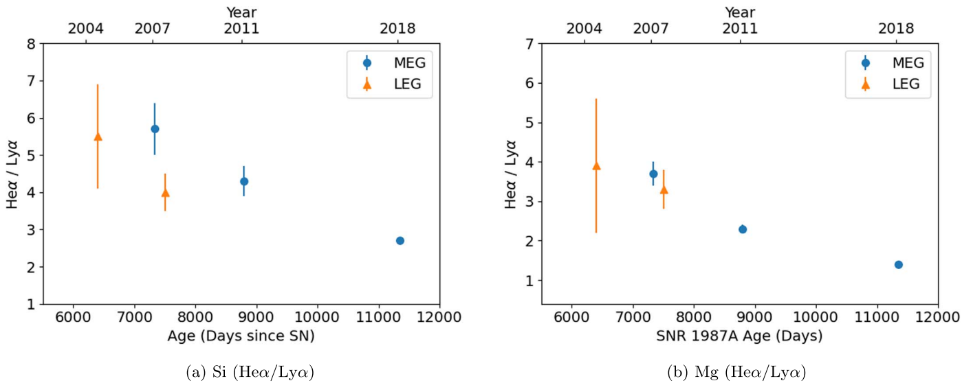
Figure 5. Temporal changes of He \alpha /Ly \alpha line-flux ratios for (a) Si (Si XIII / Si XIV) and (b) Mg (Mg XI / Mg XII) based on high-resolution Chandra grating spectra of SNR 1987A.
