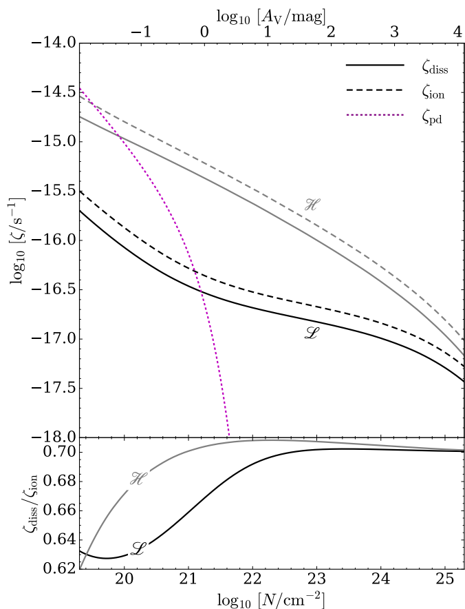
Fig. 4. Upper panel: rates of CR dissociation ( \zeta_{\text{diss}} , solid lines), CR ionisation ( \zeta_{\text{ion}} , dashed lines), and photodissociation ( \zeta_{\text{pd}} , purple dotted line) for models \mathcal{L} (black) and \mathcal{H} (grey), plotted versus the total column density of hydrogen (bottom scale) and visual extinction (top scale). Lower panel: ratio \zeta_{\text{diss}}/\zeta_{\text{ion}} for the two models.
