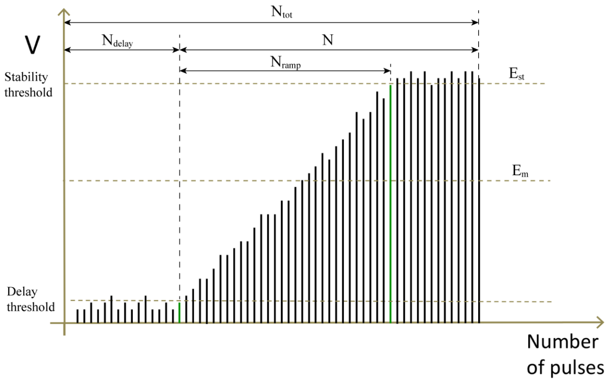
Figure 2 Laser pulsed emission trend for PRR=20 kHz and PI%=100%
