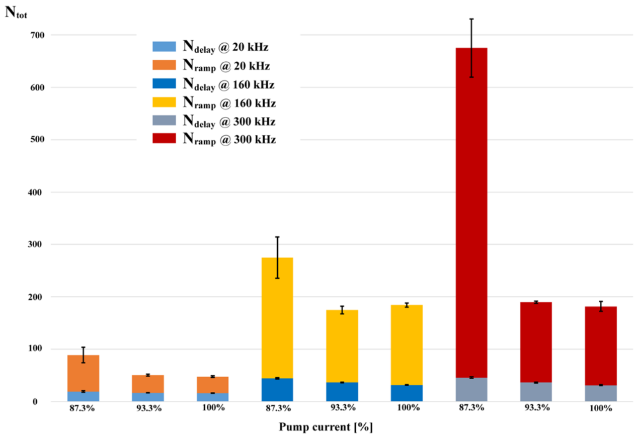
Figure 3 Ramped emission characteristics as function of laser source parameters.
