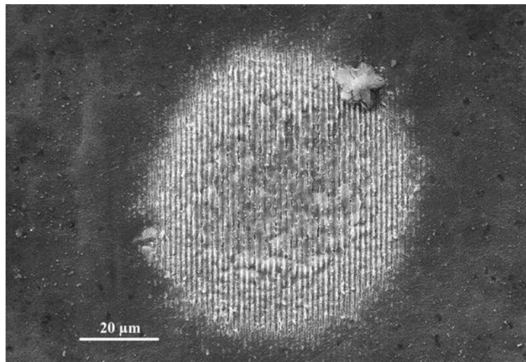
Figure 9 Laser treated spot characterized by E_{st}=20.0 \mu\text{J} , \Delta z=2 \text{ mm} , N_{tot}=80 and \theta=26^\circ
