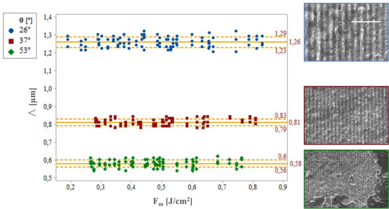
Figure 10 Measured period as a function of average fluence
