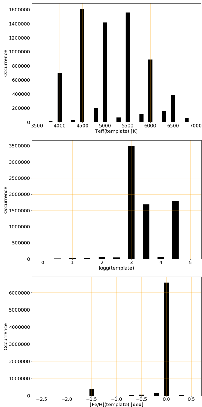
Fig. A.1. Top panel: distribution of the effective temperatures of the templates. Middle panel: distribution of the surface gravities of the templates. Bottom panel: distribution of the metallicities of the templates.
