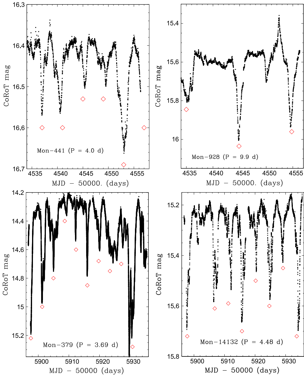
Figure 18. Light curves for four NGC 2264 CTTS whose light curves show periodic flux dips that are sometimes broad and sometimes narrow. The red diamonds mark the location of the periodic, usually narrow flux dips—in each case, placing the first diamond near the bottom of the first dip, then spacing the other diamonds by multiples of the period we have determined. We and McGinnis et al. (2015) include these stars with the classic AA Tau group, and they are shown as red circles with inscribed red plus signs in Figure 3, though their sometimes narrow flux dips suggest a link with the stars of Table 1.
