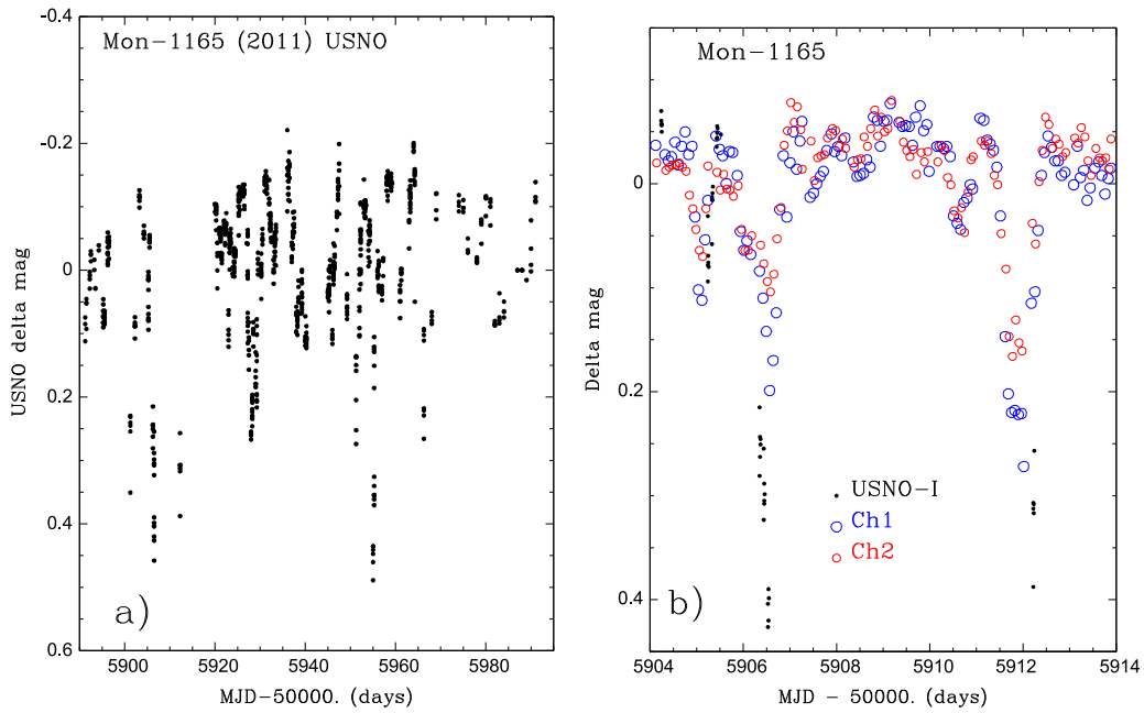
Figure 9. (a) USNO I -band light curve for Mon-1165; flux dips with depths up to about 0.4 mag appear to be present. (b) Overlay of the IRAC and USNO light curve for Mon-1165, with relatively good data in all three bands for the flux dip near MJD 55907.
