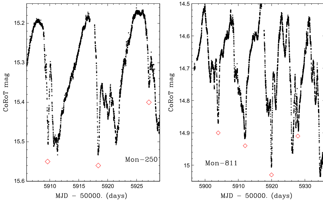
Figure 17. View of a portion of the CoRoT light curve for two AA Tau analogs, Mon-250 and Mon-811, highlighting in each light curve several narrow flux dips that are spaced in time at the period defined by the broad-flux dips. The red diamonds mark the location of the narrow flux dips. The periods are P = 8.75 days and 8.0 days, respectively.
