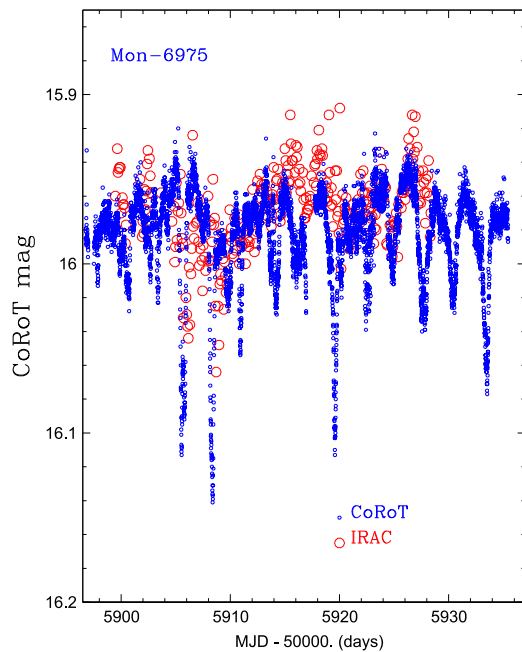
Figure 11. Overlay of the CoRoT and IRAC light curves for Mon-6975; a zero-point shift has been added to the IRAC magnitudes so they approximately align with the CoRoT data. The two strongest CoRoT flux dips have counterparts in the IRAC light curve, and there is moderate correlation in the structure of the rest of the two light curves.
