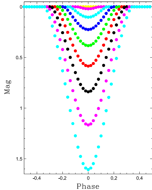
Figure 24. Model flux dips for a disk warp of fixed height and extent, where the inclination of our line of sight is varied from 65 (yellow) to 75 (light blue, at bottom) degrees in steps of 1:25. The model used is that from Bouvier et al. (1999), with the disk parameters that were appropriate to AA Tau— h_{\max} = 2.7 R_{\text{star}} , inner disk radius R_i = 8.8 R_{\text{star}} , and \phi = \pm 180^\circ .
