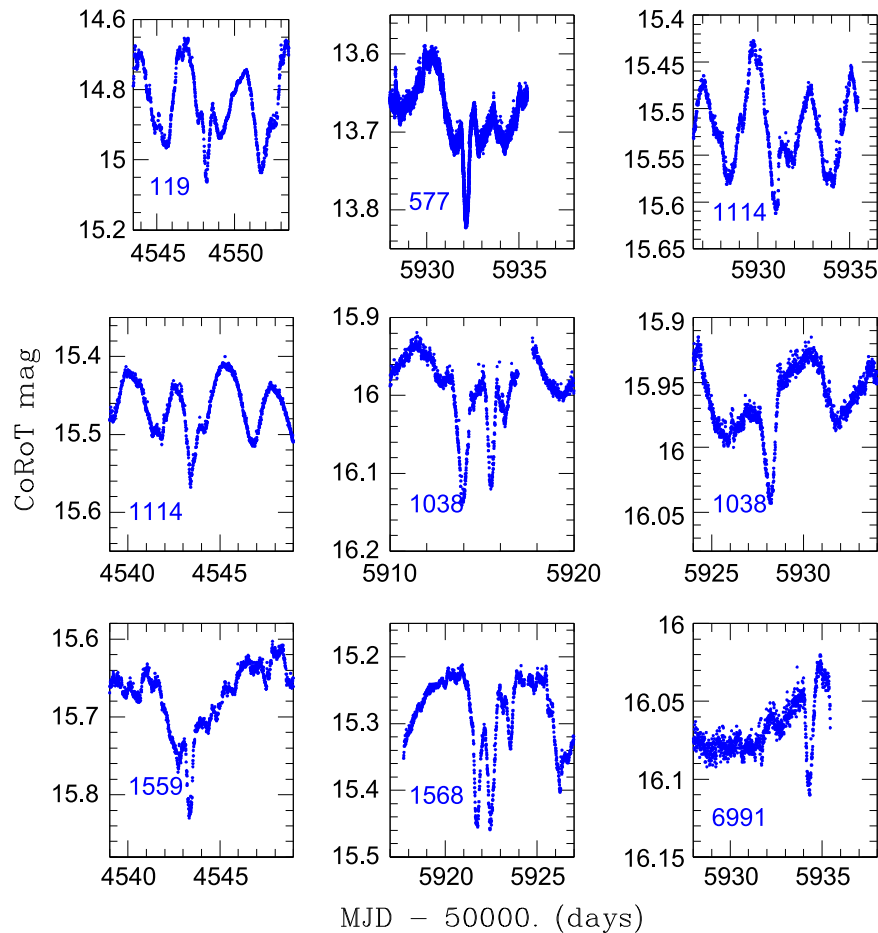
Figure 19. Isolated, short-duration flux dips found in the light curves of NGC 2264 CTTSs, for stars with only one or a few such events per CoRoT campaign—and hence for stars not previously included in our variable extinction classes. Biographical data for these stars are provided in the Appendix (Table 5).
