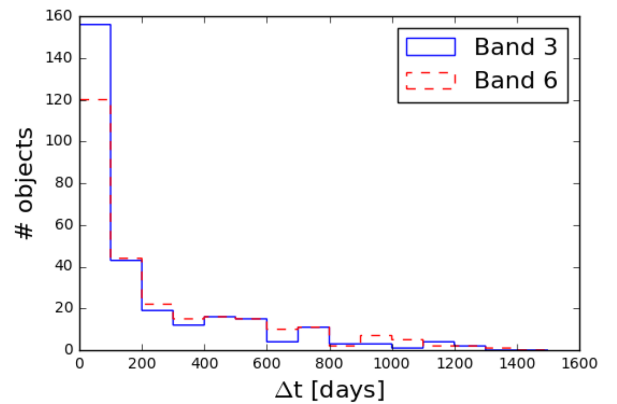
Figure 7. Distributions of the rest-frame timespans of source observations (i.e. \Delta t = [t_{last\ observation} - t_{first\ observation}] / [1 + z] ) in ALMA band 3 (solid blue line) and in band 6 (dashed red line). We only considered sources having redshift measurements and \geq 2 observations.
