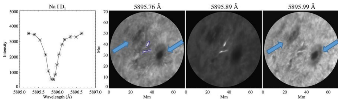
Figure 6: (Adapted from Kuridze et al. 2016). Left: IBIS Na I D1 line profile of a quiet solar region. Asterisks show the spectral positions selected for the IBIS line scan. The full black line shows the mean spectrum averaged over the field of view (FOV) of the quiet Sun. Right: Na I D1 wing and core images at selected wavelength positions. The blue contours show the upper and lower flare ribbons analyzed in the paper. Contours indicate the 50% level of the intensity maximum. The arrows indicate the main sunspots visible in the wings of the spectral line and forming the bipolar AR.
