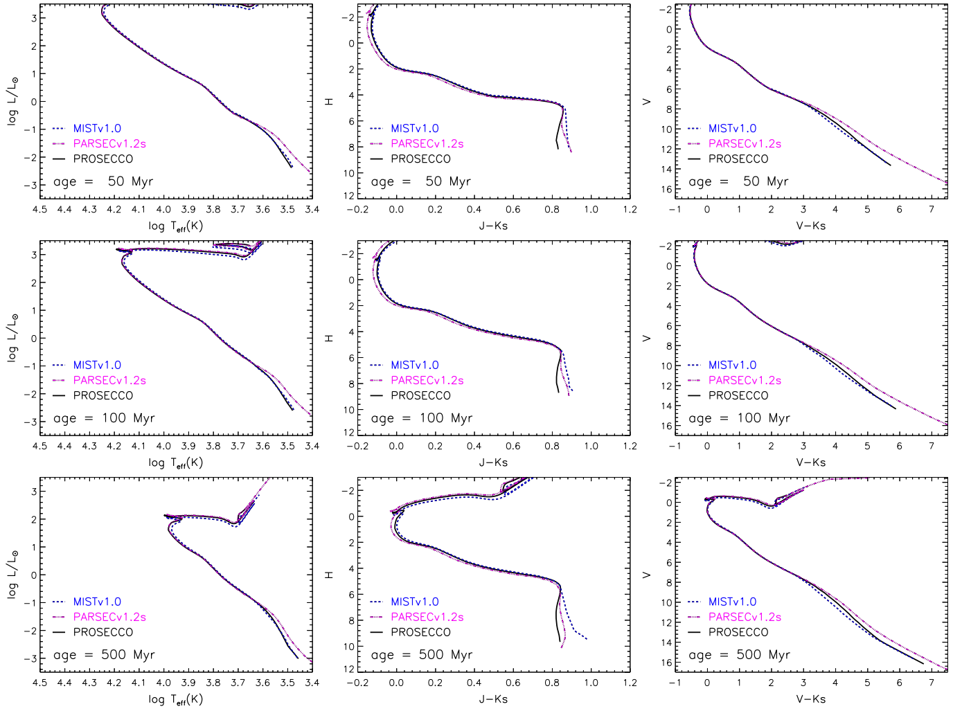
Fig. A.1. Comparison among 50, 100 and 500 Myr isochrones from the selected sets in the HR diagram and in various CM diagrams. MISTv1.0= MESA isochrones by Choi et al. (2016); Dotter (2016), PARSECv12.s= PARSEC isochrones in the PARSEC 1.2S version (Chen et al. 2014), PROSECCO= isochrones specifically calculated for the present work; see text.
