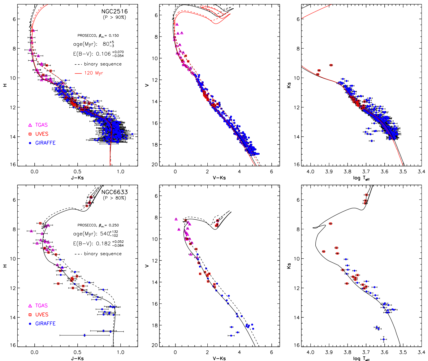
Fig. 10. As in Fig. 7 but for the clusters NGC 2516 (top panel) and NGC 6633 (bottom panel). For NGC 2516, the 120 Myr isochrone is also shown. For NGC 6633 a core overshooting parameter \beta_{ov} = 0.250 has been used.
