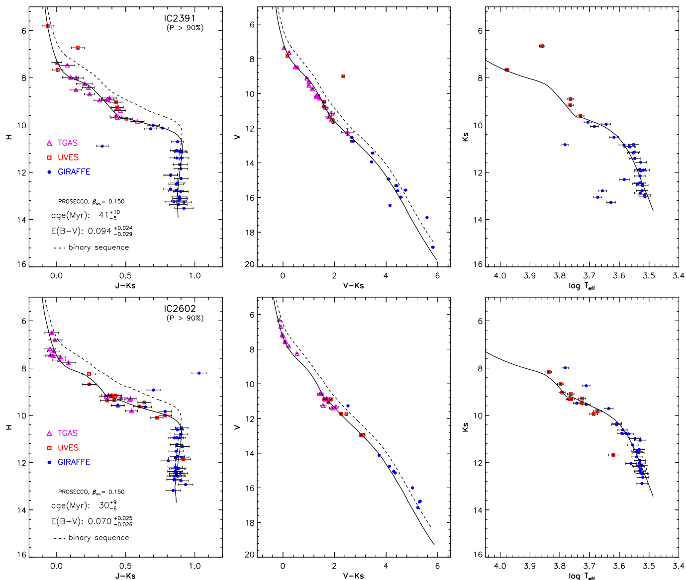
Fig. 7. Comparison between isochrones and observational data in the (J - K_s, H) , (V - K_s, V) , and (\log T_{\text{eff}}, K_s) diagrams for IC 2391 and IC 2602. Members from GES are indicated as blue full circles (GIRAFFE) and red squares (UVES), while TGAS members are plotted as magenta open triangles. Photometric data are taken from the 2MASS catalogue, AAVSO Photometric All Sky Survey (APASS) DR9 (Henden et al. 2016) and ASCC-2.5, 3rd version compilation (Kharchenko & Roeser 2009). GES iDR4 effective temperatures are adopted for the K_s versus T_{\text{eff}} diagrams. Temperatures are instead not available for the TGAS members, which are not shown in this diagram. The estimated reddening and age values are indicated in the left-hand panels - see text for more details. For both clusters, the unresolved binary sequence (with a constant mass q_{\text{bin}} = 0.8 ) is shown as a dashed line (see text).
