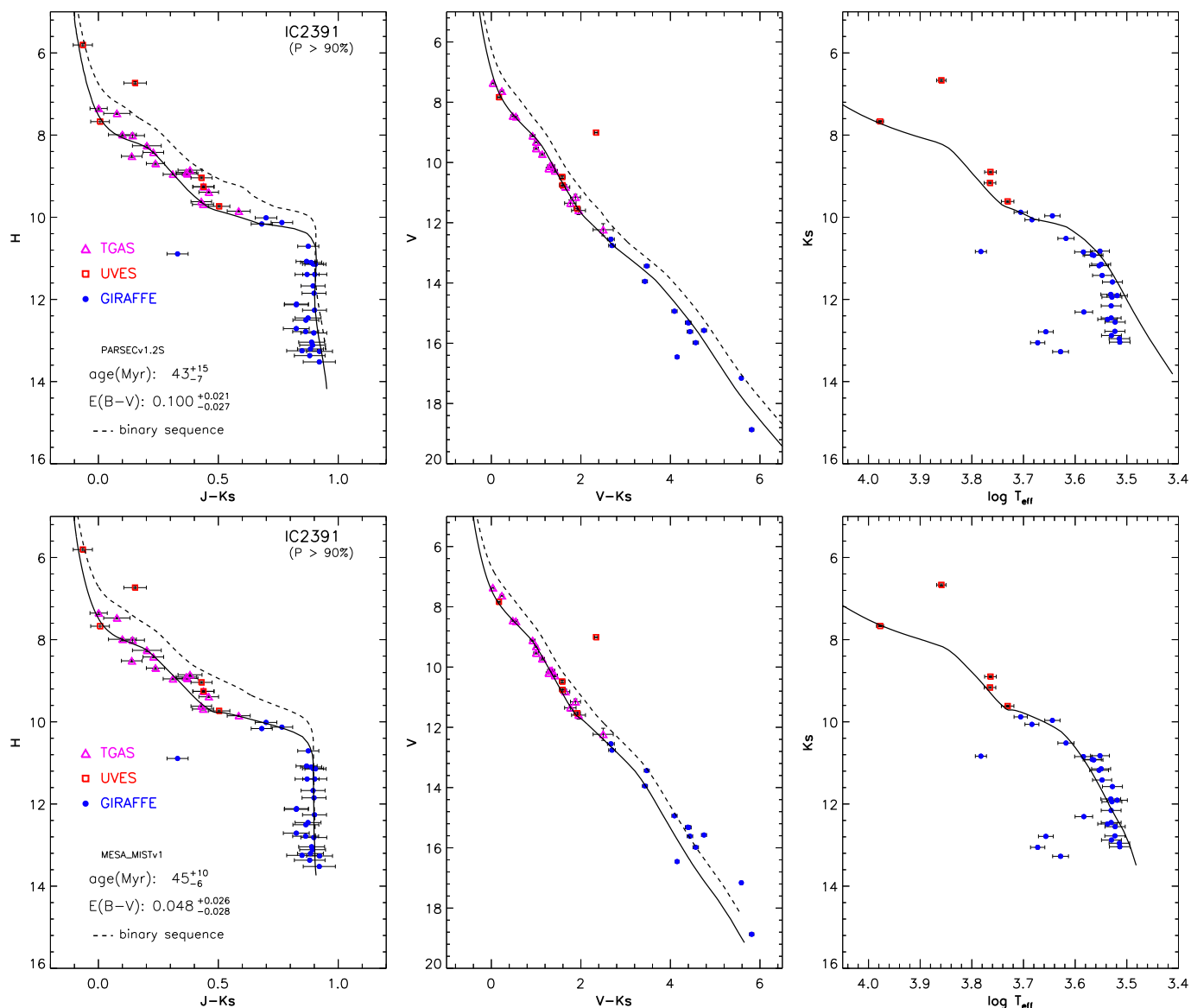
Fig. 11. As in Fig. 7 but for the cluster IC 2391 with the PARSEC (top panel) and MIST (bottom panel) isochrones.
