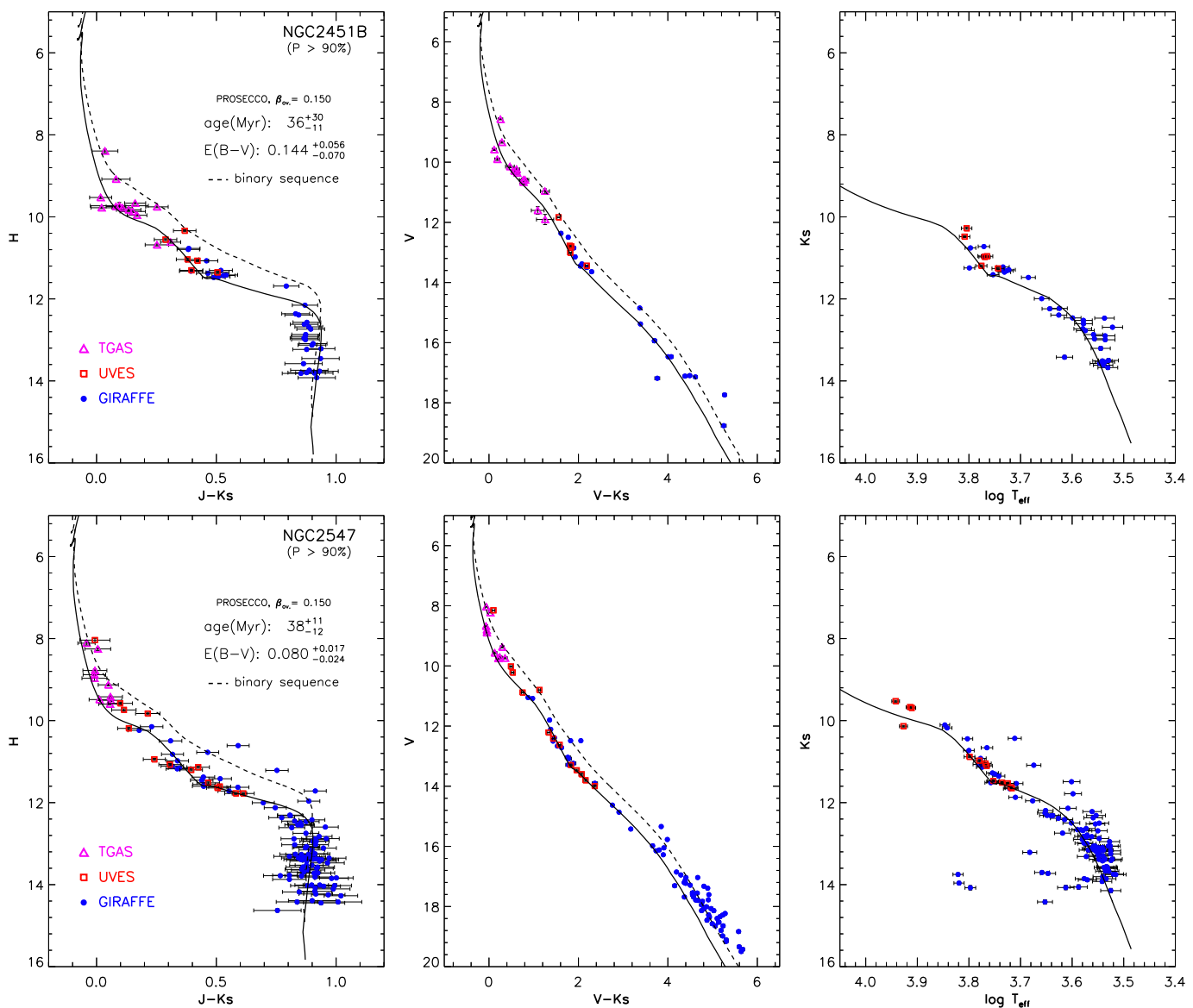
Fig. 9. As in Fig. 7 but for the clusters NGC 2451B (top panel) and NGC 2547 (bottom panel).
