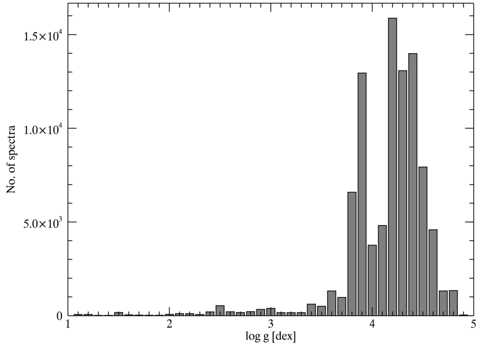
Figure 3.3: Distribution of the derived AMBRE:HARPS \log g values. This distribution peaks around the solar gravity.
