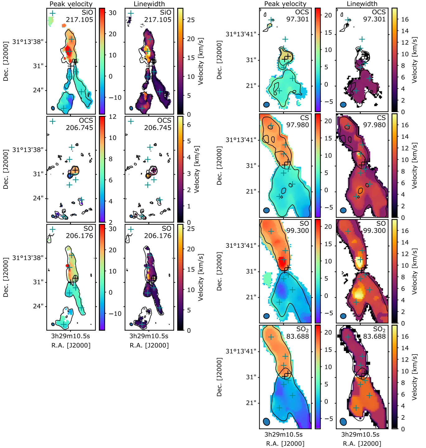
Fig. 4. Moment 1 and moment 2 maps of the SiO(5–4), OCS(17–16), and SO(6 5 –5 4 ) emission observed at “high”, 1'', angular resolution ( left panels ) and of the OCS(8–7), SO(3 2 –2 1 ), CS(2–1), and SO 2 (8 1,7 –8 0,8 ) emission at “low”, 2–4'', resolution ( right panels ). Contours represent the 3 \sigma level. Black crosses represent the position of the 4A1 and 4A2 sources of the IRAS4A binary system. Green crosses represent the position of the SiO(5–4) emission peaks along the outflows.
