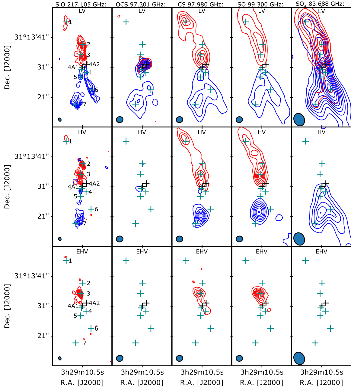
Fig. A.1. Channel maps of the main sulfurated isotopologues observed at low ( \sim 2-4'' ) resolution for three velocity ranges: low-velocity LV ( -10, +5 ) and ( +10, +25 ) \text{km s}^{-1} , high-velocity HV ( -20, -11 ) and ( +26, +40 ) \text{km s}^{-1} , and extremely-high-velocity EHV ( -35, -21 ) and ( +41, +55 ) \text{km s}^{-1} .
