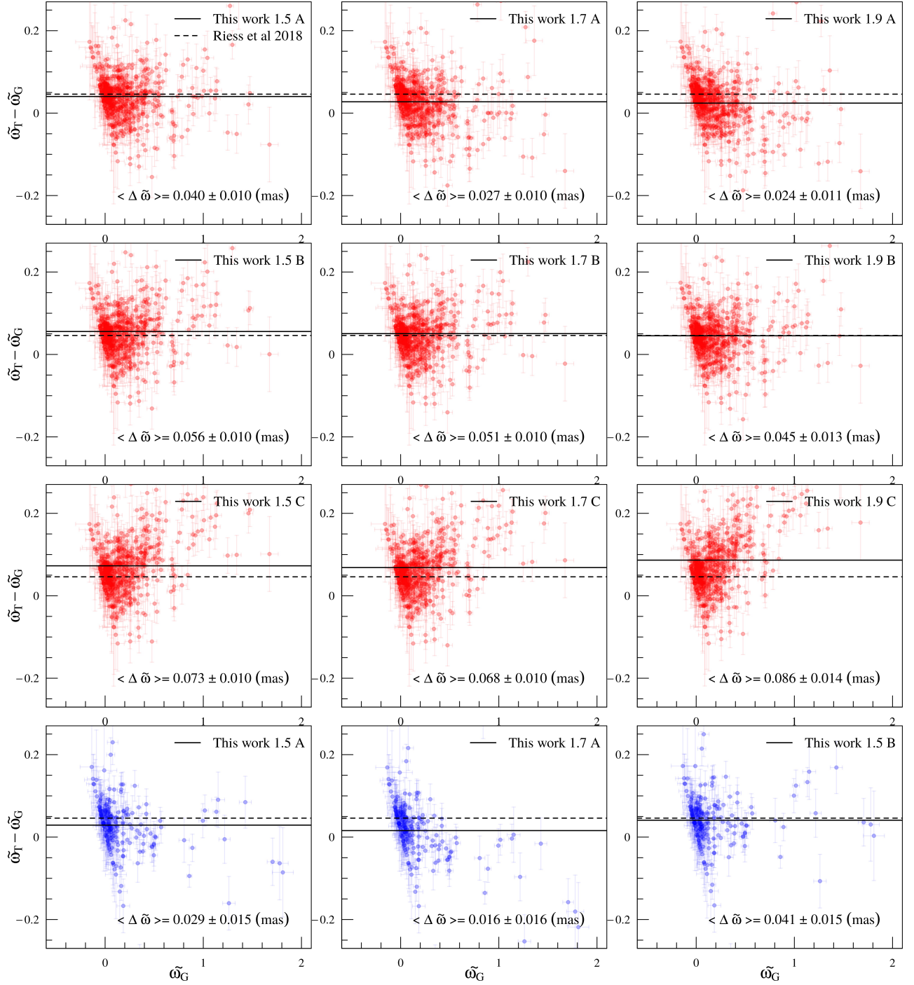
Figure 11. Parallax difference \tilde{\omega}_T - \tilde{\omega}_G for F (red points) and FO (blue points) Galactic Cepheids as a function of Gaia DR2 parallax \tilde{\omega}_G .
