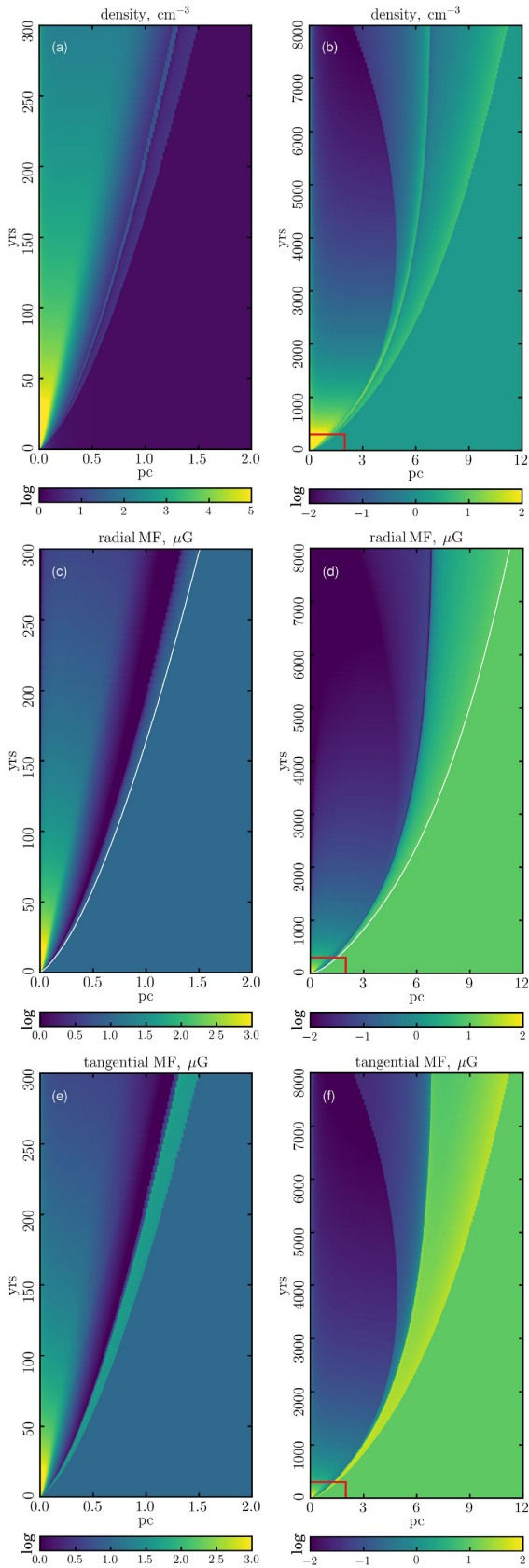
Figure 11. The same as in Fig. 10 for SNIC model.
