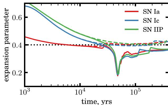
Figure 15. Evolution of the expansion parameter m for the forward shock from the early stages up to a well-developed radiative stage. Dashed lines correspond to the same models but in completely adiabatic regime when the radiative losses are switched off artificially.
