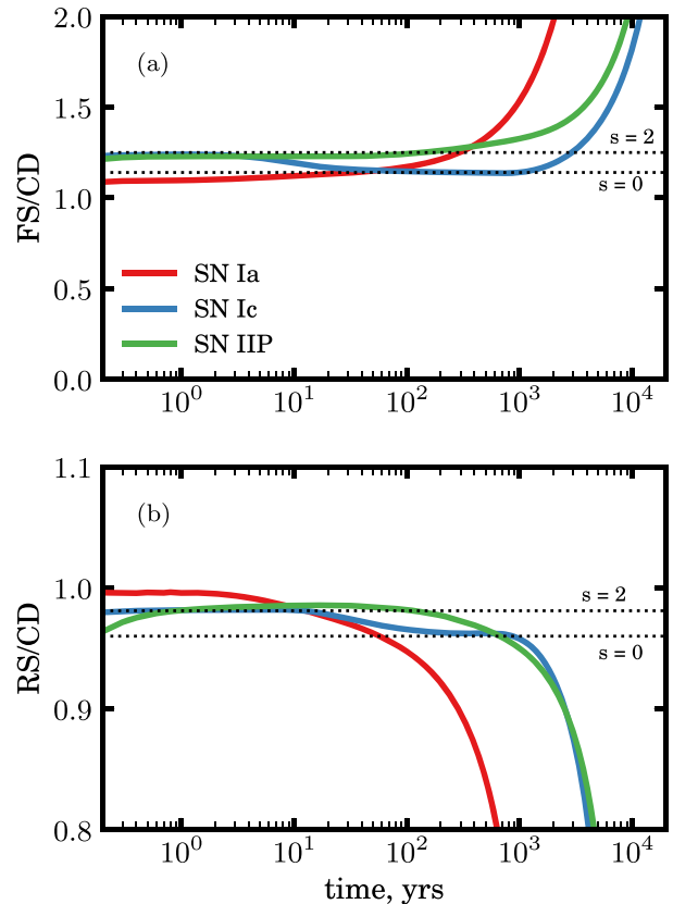
Figure 4. Evolution of the ratio of the radii derived from the simulations (solid lines): FS/CD (a) and RS/CD (b). Dotted lines are theoretical predictions from Chevalier (1982a) model for n = 9 ( s = 2 and s = 0 ). Theoretical line for n = 11 , s = 2 is not shown because of its proximity to the line for n = 9 .
