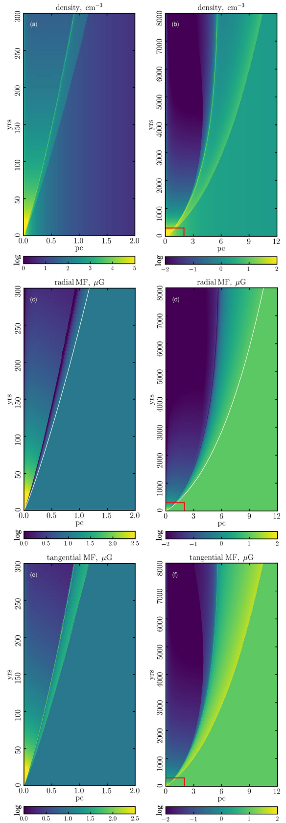
Figure 12. The same as in Fig. 10 for SNIIP model.
