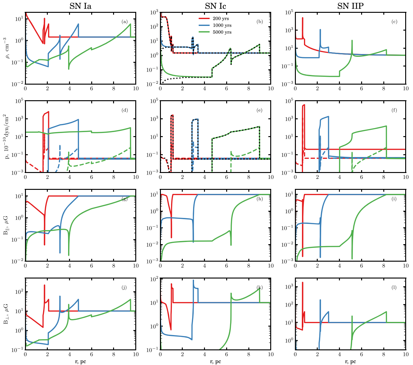
Figure 8. Radial profiles of density (top row), pressure (second row), radial MF (third row), and tangential MF (bottom row) for different SN explosion models at 200 (red line), 1000 (blue line), and 5000 yr (green line). The dashed line on pressure plots corresponds to the tangential MF pressure. All the lines for density and pressure are taken from the models with the tangential MF. Dots for the SN Ic model represent the same profiles for the radial MF.
