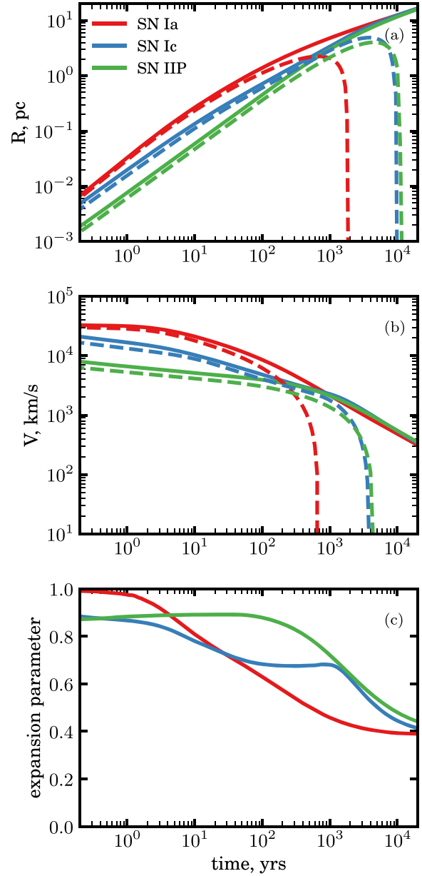
Figure 2. Dynamics of the remnants of different supernovae models (represented by different colours): evolution of the radius (a), velocity (b) of the forward (solid lines) and reverse (dashed lines) shocks as well as evolution of the expansion parameter m for the forward shock (c).
