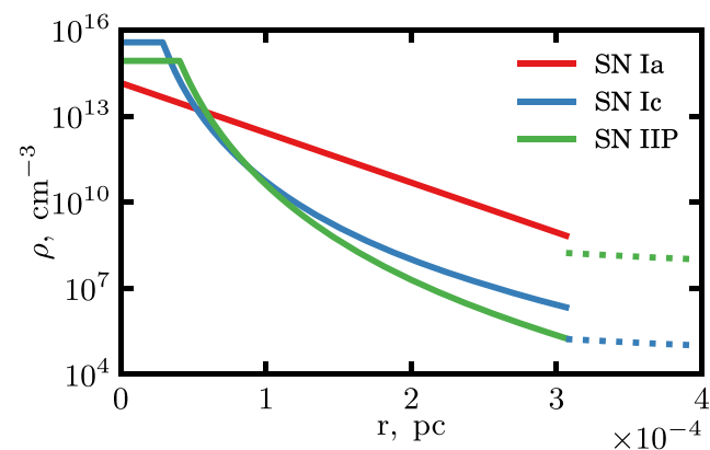
Figure 1. Radial density profiles for supernova ejecta (solid) and CSM bubbles (dotted) in the vicinity of the supernova at t_0 = 0.01 yr for our three explosion models. SNR after type-Ia event evolves in a uniform ISM with n_0 = 1 \text{ cm}^{-3} (not shown here).
