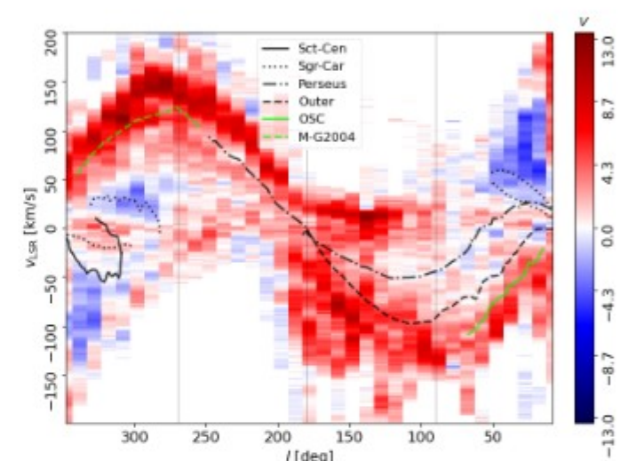
Fig. A.4: Same as Fig. 7, but for tile sizes 20^\circ \times 20^\circ \times 1.29 \text{ km s}^{-1} .
