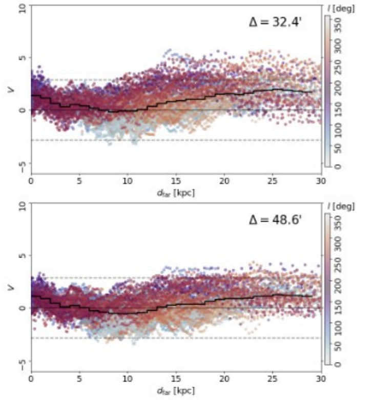
Fig. A.8: Same as Fig. 4, but for 32.4' and 48.6' FWHM derivative kernels, shown in the top and the bottom panels, respectively.
