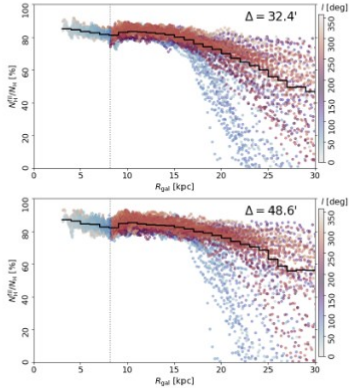
Fig. A.9: Same as Fig. 12, but for 32.4' and 48.6' FWHM derivative kernels, shown in the top and the bottom panels, respectively.
