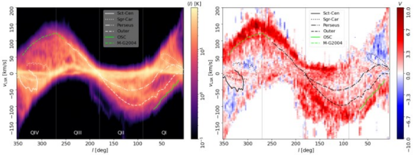
Fig. 1: Longitude-velocity ( lv ) diagrams of the mean intensity ( \langle I , left) and the filament orientation quantified by the projected Rayleigh statistic ( V , right). Each of the pixel elements in the diagrams corresponds to a 3^\circ \times 20^\circ \times 1.29 \text{ km s}^{-1} velocity channel map centered on b = 0^\circ , which we call tile throughout this paper. These results correspond to the Hessian analysis performed using an 18' FWHM derivative kernel. Values of V > 0 (red) or V < 0 (blue) indicate a preferential orientation of the filaments parallel, \theta = 0^\circ , or perpendicular, \theta = 90^\circ , to the Galactic plane. The 3\sigma statistical significance for these two orientations corresponds to V > 2.87 or V < -2.87 , respectively. The overlaid curves correspond to the main spiral arms features presented in Reid et al. (2016), the outer Scutum-Centaurus arm (OSC, Dame & Thaddeus 2011), and the extended outer arm (M-G2004, McClure-Griffiths et al. 2004).
