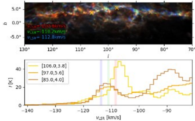
Fig. 19: HI emission ( top ) and selected spectra toward filamentary structures ( bottom ). The spectra correspond to the positions indicated by the crosses in the upper panel. The colored vertical bars in the bottom panel correspond to the three velocity channels presented in the corresponding colors in the top panel.
