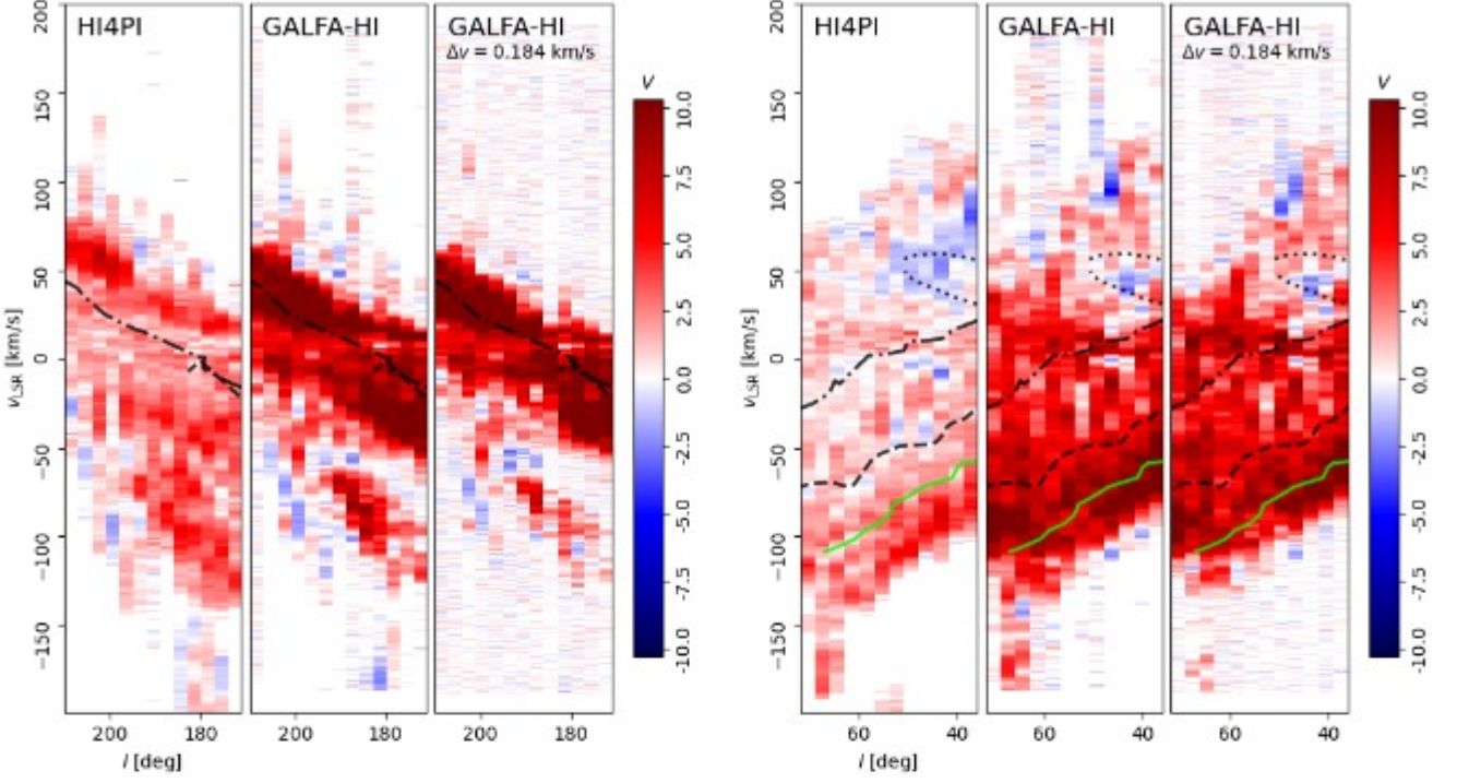
Fig. 14: Longitude-velocity ( lv ) diagrams of the filament orientation quantified by the projected Rayleigh statistic ( V , right) in the two portions of the Galactic plane covered in the range |b| \leq 10^\circ by both HI4PI and GALFA-HI. The GALFA-HI observations were analyzed at 1.29 and 0.184 \text{km s}^{-1} resolution using a 5' FWHM derivative kernel. The curves correspond to the same spiral arm features introduced in Fig. 1.
