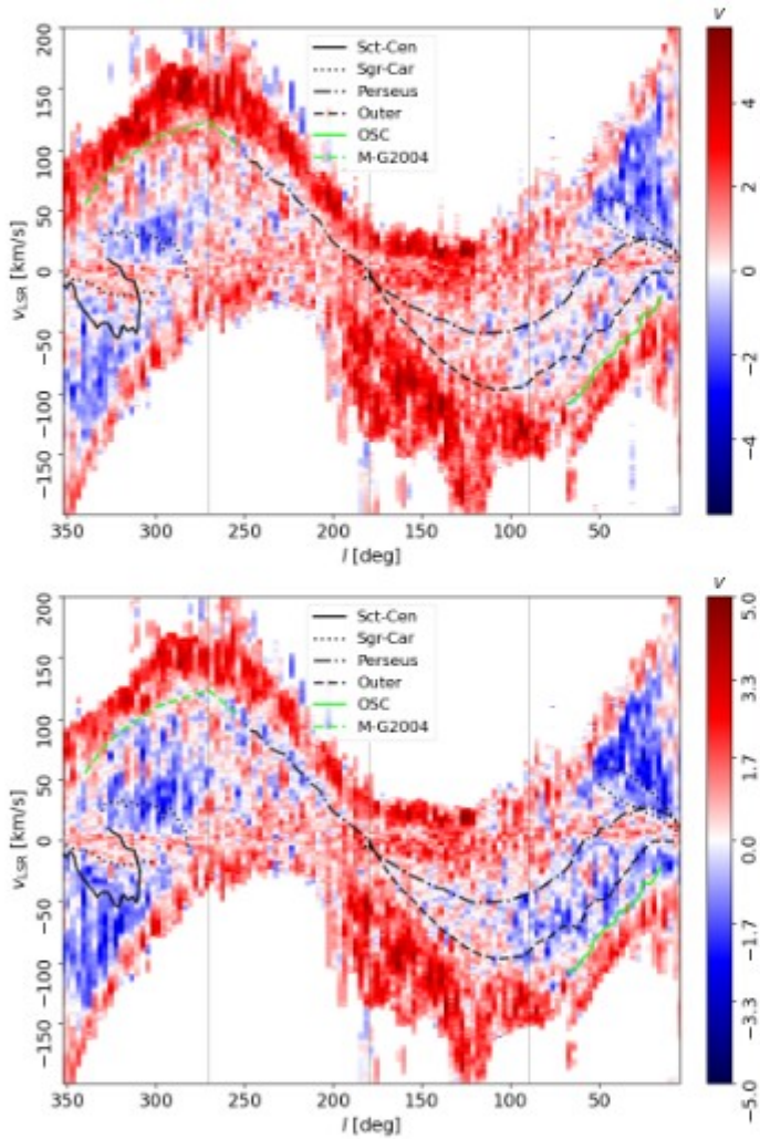
Fig. A.7: Same as Fig. A.3, but for 3^\circ \times 20^\circ \times 1.29 \text{ km s}^{-1} tiles analyzed using 32.4' and 48.6' FWHM derivative kernels, shown in the top and the bottom panels, respectively.
