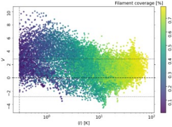
Fig. 2: Mean HI emission intensity ( \langle I \rangle ) and projected Rayleigh statistic ( V , Eq. 4) for the 3^\circ \times 20^\circ \times 1.29 \text{ km s}^{-1} tiles. The colors indicate the tile percentage covered by the filamentary structures selected following the criteria described in Sec. 3.2. The horizontal dotted lines show V = \pm 2.87 , which indicate the 3\sigma significance in the preferential orientation parallel, \theta = 0^\circ , or perpendicular, \theta = 90^\circ , to the Galactic plane, respectively. The vertical dashed line indicates the intensity threshold.
