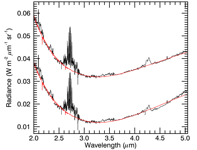
Figure 3. VIRTIS-H spectrum acquired on 13 September from 13.7125 to 13.7968 h UT. In the top spectrum, radiance values measured in the range 4.2 – 5 \mu\text{m} were corrected as described in Sect. 3.2, with s=0.2 . This correction is not applied in the bottom spectrum. Overplotted, in red, are the best model fits.
