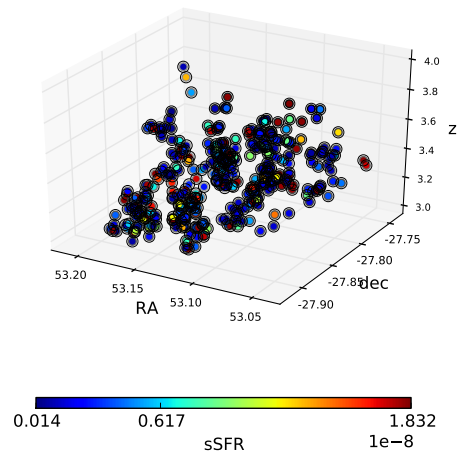
Fig. B.7. Same as Fig. B.1 for the overdensity detected at z = 3.17 in the CDFS.
