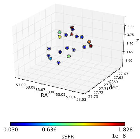
Fig. B.13. Same as Fig. B.1 for the overdensity detected at z = 3.69 in the CDFS.
