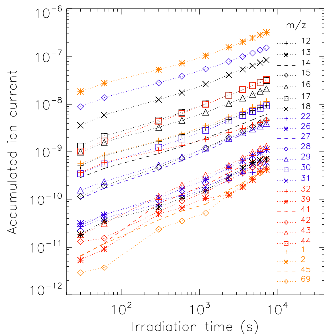
Figure 3. Accumulated quadrupole mass spectrometer signal as a function of the irradiation time for the photo-desorbing species detected during irradiation in the BBs experiment (see Table 1).
