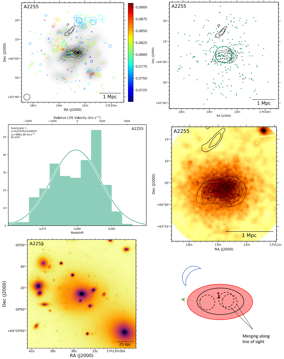
Figure 21. Top left: DS-test over red sequence R-band luminosity distribution with linearly space white contours. The black contours show the 350 MHz WSRT contours (Pizzo & de Bruyn 2009). Top right: Subcluster membership of spectroscopic cluster members assigned with our GMM analysis. The same WSRT contours (solid) and red sequence luminosity contours (dashed) are depicted. The small projected separation and low spectroscopic survey density likely contributes to a single halo model being preferred. Middle left: Subcluster redshift histograms with colors matching the image at the top right. Middle right: 42 ks XMM image with the same WSRT radio contours (solid) and red sequence luminosity contours (dashed). The relic at the northeast and the disturbed ICM are suggestive of a merger between at least three subclusters. Bottom left: 150 kpc cutout of the Subaru/SuprimeCam R-band image centered on the cluster BCG in the western half of the cluster. The second BCG apparent in the image has a \sim 2000 \text{ km s}^{-1} line of sight velocity difference, which is suggestive of a merger along the line of sight. Bottom right: Preferred merger scenario. The elongation of the X-ray surface brightness suggests a second plane of the sky merger component in addition to the line of sight merger. We do not make a prediction of which subclusters merged to launch the radio relic. We can not rule out further complications in this system.
