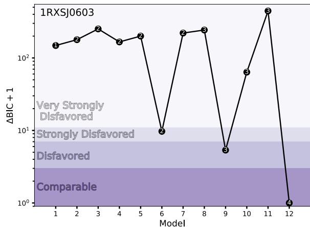
Figure 4. Bayesian Information Criterion scores relative to the most economical model for twelve 3D (RA, DEC, z ) Gaussian Mixture Models fit to the 242 spectroscopic cluster member galaxies of 1RXSJ0603. The numbers in the black points indicate the number of subclusters included in a given model. The shaded regions roughly denote how a given model compares with the lowest BIC score (Kass & Raftery 1995). The most economical fit is a four component model (see Table 3 and 4). An analogous plot is not presented for each cluster; however, the \Delta BIC scores are presented in Table 4.
