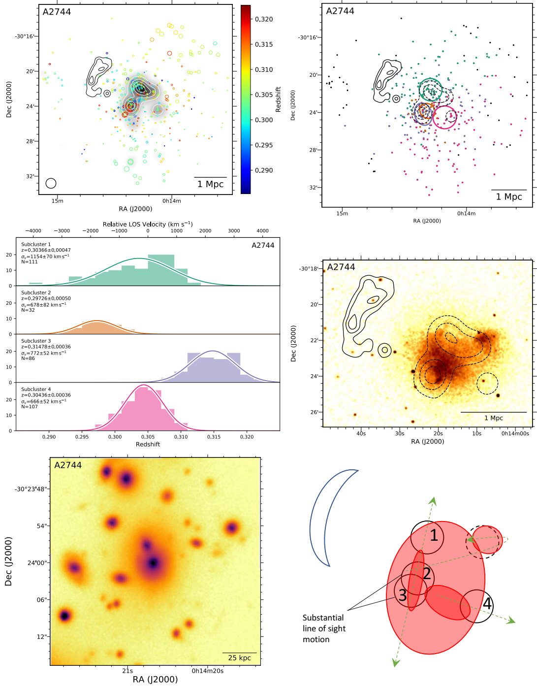
Figure 24. Top left: DS-test over red sequence Subaru/SuprimeCam R-band luminosity distribution with linearly spaced white contours. The black contours show the 325 MHz GMRT contours (Venturi et al. 2013). Top right: Subcluster membership of spectroscopic cluster members assigned with our GMM analysis. The same GMRT contours (solid) and red sequence luminosity contours (dashed) are depicted. Middle left: Subcluster redshift histogram with colors matching the image at the top right. Middle right: 132 ks Chandra image with the same GMRT radio contours (solid) and red sequence luminosity contours (dashed). Bottom left: 150 kpc cutout of the Subaru/SuprimeCam R-band image centered on the cluster BCG in subcluster 2. Bottom right: Preferred merger scenario. A2744 is the most complex merger in our sample. The core of the cluster (subclusters 2 and 3) has been studied in detail as a HST Frontier Field and has a substantial line of sight motion. Subclusters 1 and 4 have been stripped of their ICM suggesting post merger scenarios. Finally, a fifth subcluster with an associated ICM further from the cluster than the galaxies suggests a ram-pressure slingshot type scenario.
