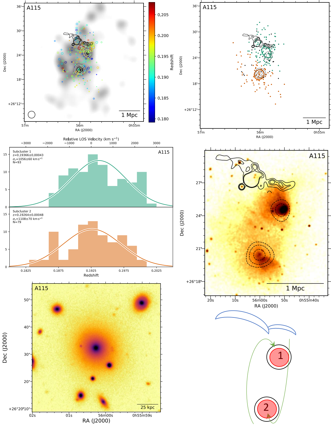
Figure 10. Top left: DS-test over red sequence i -band luminosity distribution with linearly space white contours. The black contours show the 1.4 GHz VLA contours (Govoni et al. 2001b). Top right: Subcluster membership of spectroscopic cluster members assigned with our GMM analysis. The same VLA contours (solid) and red sequence luminosity contours (dashed) are depicted. Middle left: Subcluster redshift histograms with colors matching the image at the top right. Middle right: 376 ks Chandra image with the same VLA radio contours (solid) and red sequence luminosity contours (dashed). The glancing merger scenario is clear from the swirling stream of X-ray emission. Bottom left: 150 kpc cutout of the Subaru/SuprimeCam image centered on the BCG of subcluster 2. Bottom right: Schematic of preferred merger scenario showing a large impact parameter merger and spiraling motion in the observed state.
