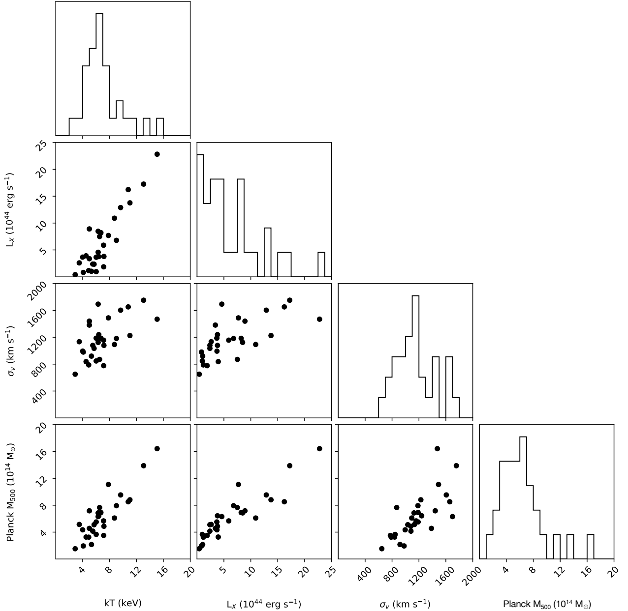
Figure 42. Relationships between four global measures for 29 merging clusters. The clear positive correlation between each suggests that, measuring these values gives a first order understanding of the mass of a merging system. Furthermore, with further lensing and dynamical study, we may understand why given systems have higher \sigma_v with respect to merger dynamics.
