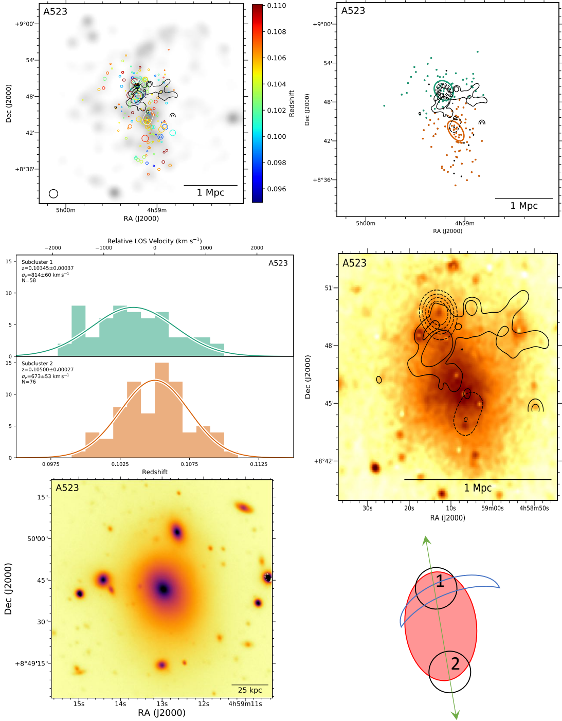
Figure 12. Top left: DS-test over red sequence r-band luminosity distribution with linearly spaced white contours. The black contours show the 1.4 GHz VLA contours (van Weeren et al. 2011b). Top right: Subcluster membership of spectroscopic cluster members assigned with our GMM analysis. The same VLA contours (solid) and red sequence luminosity contours (dashed) are depicted. Middle left: Subcluster redshift histograms with colors matching the image at the top right. Middle right: 30 ks Chandra image with the same VLA radio contours (solid) and red sequence luminosity contours (dashed). A bimodal merger scenario is evident, but the radio emission is not clearly tracing a potential merger induced shock between subclusters 1 and 2. Bottom left: 150 kpc cutout of the Subaru/SuprimeCam r-band image centered on the BCG of subcluster 1. Bottom right: Proposed merger scenario. A523 is a clean bimodal merger with a difficult to interpret radio feature that has been debated in the literature.
