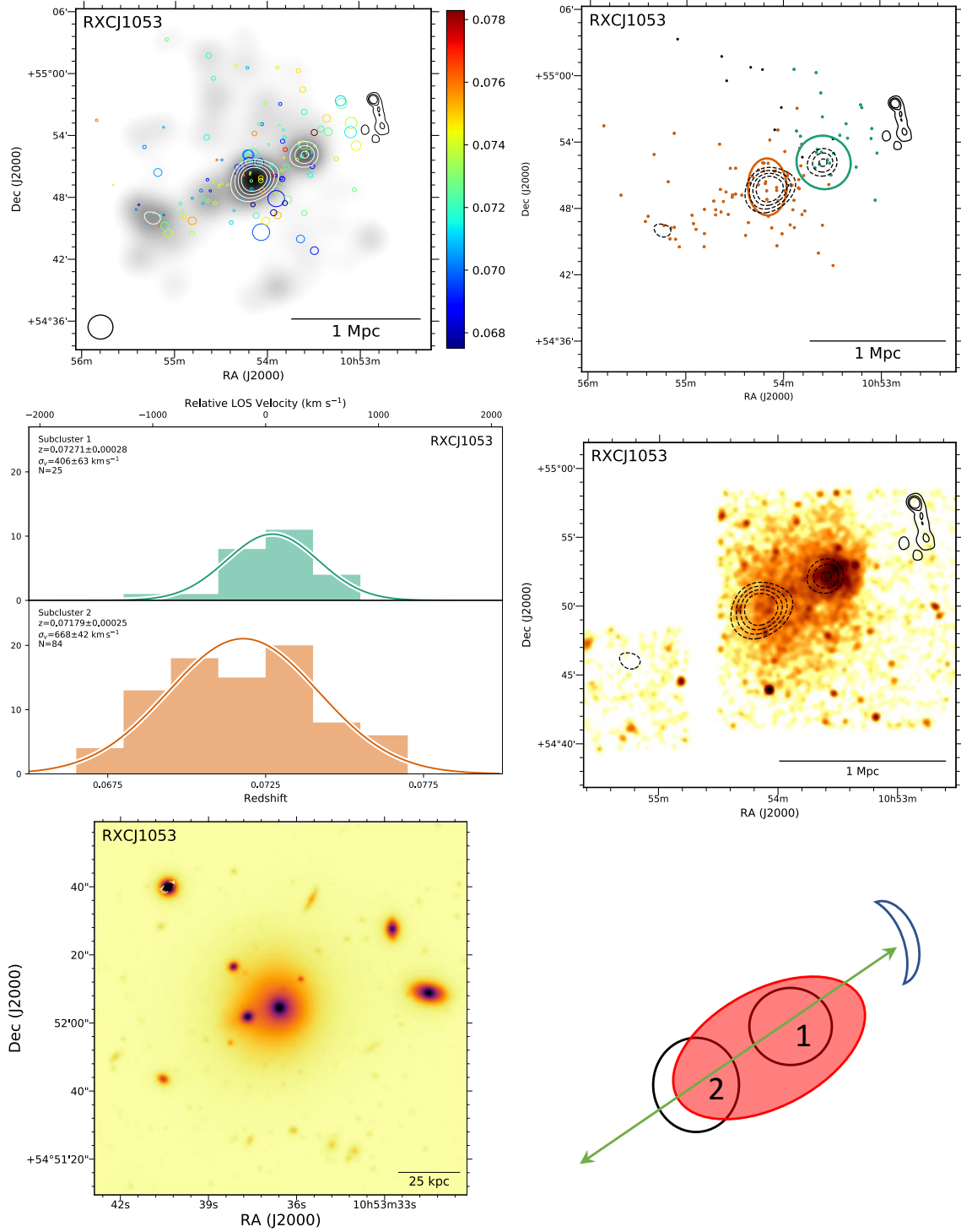
Figure 32. Top left: DS-test over red sequence Subaru/SuprimeCam r-band luminosity distribution with linearly space white contours. The black contours show WSRT 1382 MHz contours (Bonafede et al. 2014). Top right: Subcluster membership of spectroscopic cluster members assigned with our GMM analysis. The same WSRT contours (solid) and red sequence luminosity contours (dashed) are depicted. Middle left: Subcluster redshift histogram with colors matching the image at the top right. Middle right: 31 ks Chandra image with the same WSRT radio contours (solid) and red sequence luminosity contours (dashed). Bottom left: 150 kpc cutout of the Subaru r-band image centered on the cluster BCG in subcluster 1. Bottom right: Preferred merger scenario. The two subclusters and radio relic are aligned with the extended X-ray emission. Most of the mass appears to be associated with subcluster 2; however, the X-ray emission is associated with subcluster 1, which is perhaps a signature of a cool-core remnant. Deeper X-ray observations are necessary to reveal the nature of the ICM.
