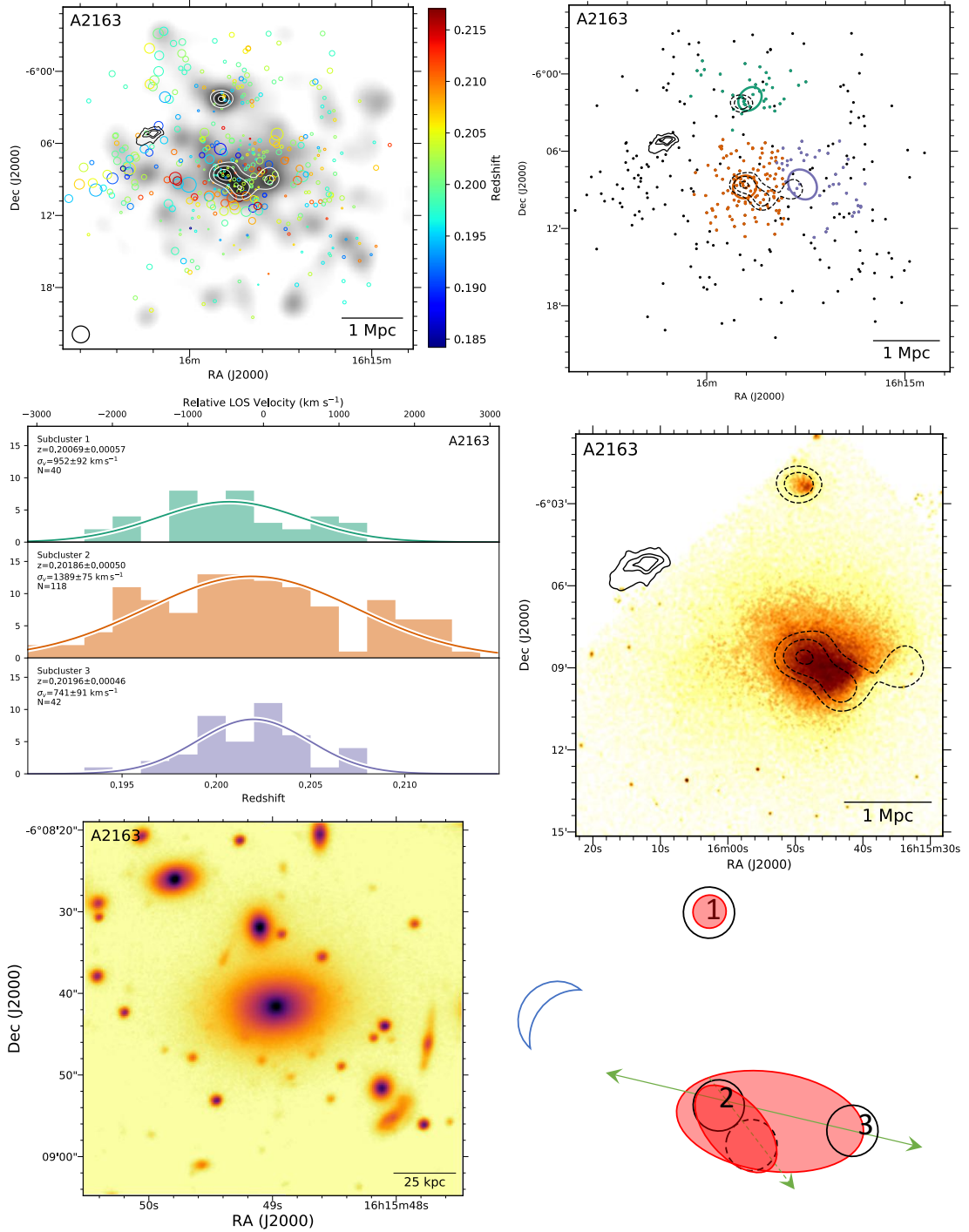
Figure 20. Top left: DS-test over red sequence R-band luminosity distribution with linearly space white contours. The black contours show the 1.4 GHz VLA contours (Feretti et al. 2001). Top right: Subcluster membership of spectroscopic cluster members assigned with our GMM analysis. The same VLA contours (solid) and red sequence luminosity contours (dashed) are depicted. The small projected separation between the two apparent subclusters comprising subcluster 2 likely contributes to a single halo describing this region. Middle left: Subcluster redshift histograms with colors matching the image at the top right. Middle right: 90 ks Chandra image with the same VLA radio contours (solid) and red sequence luminosity contours (dashed). The relic at the northeast and the disturbed ICM are suggestive of a merger between at least three subclusters. The northernmost subcluster 1 has yet to merge. Bottom left: 150 kpc cutout of the Subaru/SuprimeCam R-band image centered on the cluster BCG in subcluster 2. Bottom right: Preferred merger scenario. The large projected distance to the radio relic suggest an older merger. Subcluster 1 has yet to merge, and subcluster 3 has been stripped of its ICM suggesting it is post pericenter. A fourth subcluster is likely associated with the cool core remnant identified by Bourdin et al. (2011). This merger is very near core-crossing and likely contributing to the very high X-ray luminosity and SZ inferred mass.
