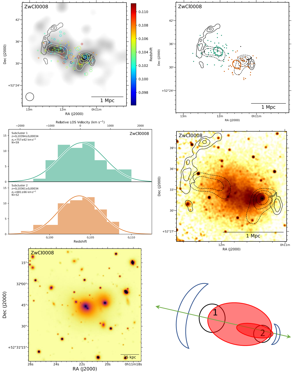
Figure 34. Top left: DS-test over red sequence Subaru/SuprimeCam r-band luminosity distribution with linearly spaced white contours. The black contours show WSRT 1382 MHz contours (van Weeren et al. 2011c). Top right: Subcluster membership of spectroscopic cluster members assigned with our GMM analysis. The same WSRT contours (solid) and red sequence luminosity contours (dashed) are depicted. Middle left: Subcluster redshift histogram with colors matching the image at the top right. Middle right: 411 ks Chandra image with the same WSRT radio contours (solid) and red sequence luminosity contours (dashed). Bottom left: 150 kpc cutout of the Subaru r-band image centered on the cluster BCG in subcluster 2. Bottom right: Preferred merger scenario. The two subclusters and radio relics are aligned with the extended X-ray emission. A ‘bullet’ like cool-core remnant and wake feature are associated with subcluster 2, which is traveling to the west. The cluster exhibits simple, bimodal geometry indicative of the Bullet Cluster.
