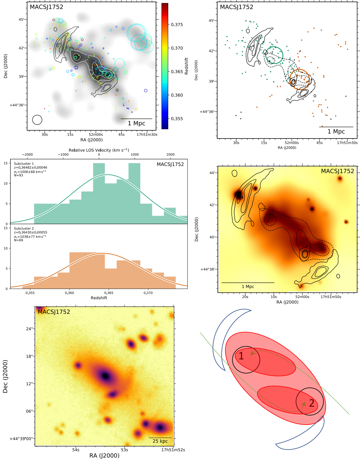
Figure 29. Top left: DS-test over red sequence Subaru/SuprimeCam i-band luminosity distribution with linearly spaced white contours. The black contours show WSRT 1.4 GHz contours (van Weeren et al. 2012a). Top right: Subcluster membership of spectroscopic cluster members assigned with our GMM analysis. The same WSRT contours (solid) and red sequence luminosity contours (dashed) are depicted. Middle left: Subcluster redshift histogram with colors matching the image at the top right. Middle right: 13 ks XMM image with the same WSRT radio contours (solid) and red sequence luminosity contours (dashed). Bottom left: 150 kpc cutout of the Subaru i-band image centered on the cluster BCG in subcluster 2. Bottom right: Preferred merger scenario. The X-ray image shows evidence for two ‘bullets’ that just missed and are beginning to orbit one another counter-clockwise. There two relics are bright and suggest a major merger despite not being head-on. The two subclusters have similar velocity dispersions and line of sight velocities suggesting the orbital plane is perpendicular to the line of sight.
