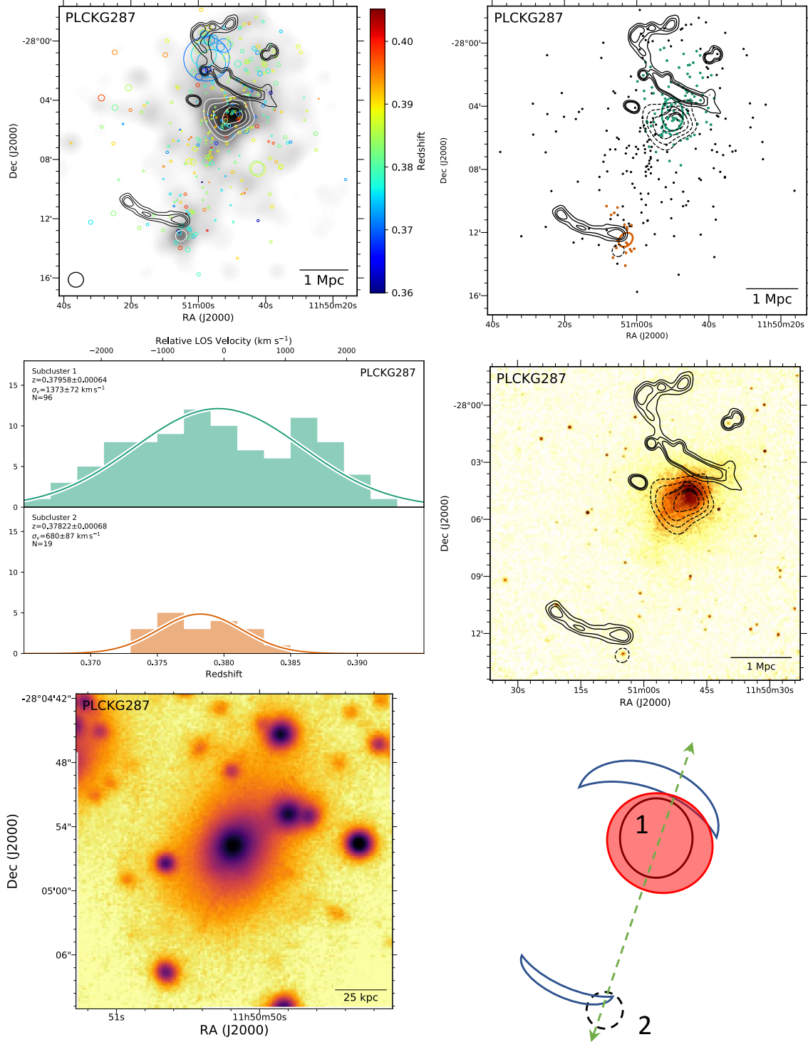
Figure 30. Top left: DS-test over red sequence Subaru/SuprimeCam r-band luminosity distribution with linearly spaced white contours. The black contours show GMRT 325 GHz contours (Bonafede et al. 2014). Top right: Subcluster membership of spectroscopic cluster members assigned with our GMM analysis. The same GMRT contours (solid) and red sequence luminosity contours (dashed) are depicted. Middle left: Subcluster redshift histogram with colors matching the image at the top right. Middle right: 200 ks Chandra image with the same GMRT radio contours (solid) and red sequence luminosity contours (dashed). Bottom left: 150 kpc cutout of the Subaru i-band image centered on the cluster BCG in subcluster 1. Bottom right: Preferred merger scenario. The merger scenario is unclear. There is evidence for a small subcluster in the south near the southern radio relic; however, it leads the relic. There is disturbed X-ray emission streaming to the south of subcluster 1, which could motivate this merger scenario. A detailed weak gravitational lensing analysis detected composite structure in subcluster 1 (Finner et al. 2017), and more complex scenarios have been proposed (Bonafede et al. 2014).
