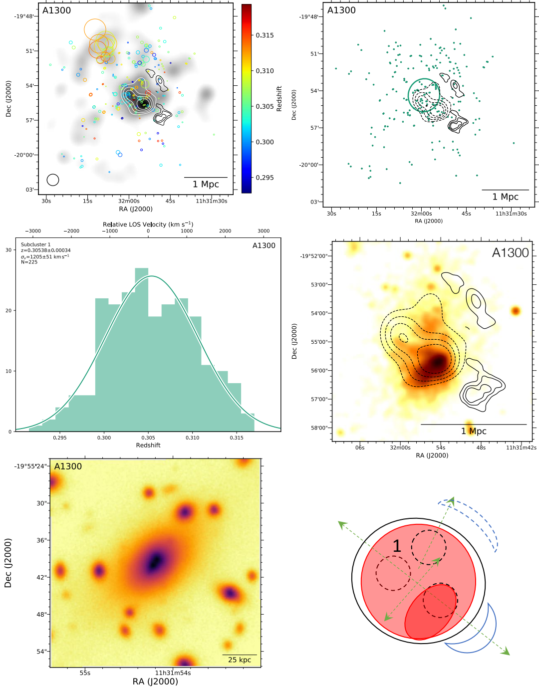
Figure 16. Top left: DS-test over red sequence r-band luminosity distribution with linearly spaced white contours. The black contours show the 325 MHz GMRT contours (Venturi et al. 2013). Top right: Subcluster membership of spectroscopic cluster members assigned with our GMM analysis. The same GMRT contours (solid) and red sequence luminosity contours (dashed) are depicted. The small projected separation and low spectroscopic survey density likely contributes to a single halo model being preferred by the BIC analysis. Middle left: Subcluster redshift histograms with colors matching the image at the top right. Middle right: 100 ks Chandra image with the same GMRT radio contours (solid) and red sequence luminosity contours (dashed). The relics and disturbed ICM are suggestive of a complex merger between at least three subclusters. Bottom left: 150 kpc cutout of the Subaru/SuprimeCam r-band image centered on the cluster BCG. Bottom right: Proposed merger scenario. A1300 is a difficult to interpret merger with likely at least three subclusters. The X-ray surface brightness morphology is suggestive of an additional merger axis associated with the an additional merger in the southwest to northeast direction. The BCG is elongated along the same axis. Inspection of the higher resolution HST RELICS images at https://www.spacetelescope.org/images/potw1745a/ show the BCG is actually composed of two luminosity peaks along this axis.
