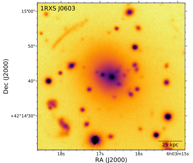
Figure 8. Subaru/SuprimeCam r-band cutout of the inner 150 \times 150 kpc of the BCG of 1RXSJ0603. A strongly lensed arc is apparent along with several light peaks within the inner region of the overall light profile. This figure, along with the 28 analogous figures in the respective following subsections will be analyzed in detail in a forthcoming paper.
