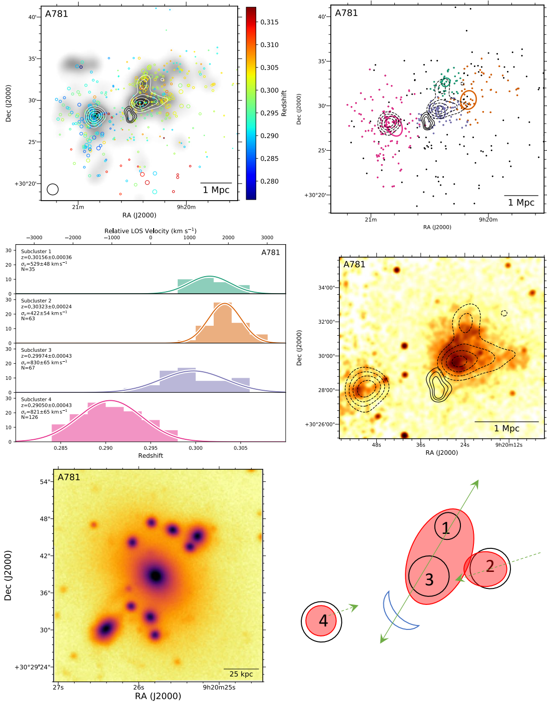
Figure 14. Top left: DS-test over red sequence i-band luminosity distribution with linearly spaced white contours. The black contours show the 325 MHz GMRT contours (Venturi et al. 2013). Top right: Subcluster membership of spectroscopic cluster members assigned with our GMM analysis. The same GMRT contours (solid) and red sequence luminosity contours (dashed) are depicted. Middle left: Subcluster redshift histograms with colors matching the image at the top right. Middle right: 48 ks Chandra image with the same WSRT radio contours (solid) and red sequence luminosity contours (dashed). The relic and disturbed ICM are suggestive of a merger between subclusters 1 and 3. Bottom left: 150 kpc cutout of the Subaru/SuprimeCam i-band image centered on the cluster BCG, which is associated with subcluster 3. Bottom right: Proposed merger scenario. The ICM is most disrupted between subclusters 1 and 3 with subcluster 2 having a less disturbed ICM coincident with its galactic light. Subcluster 4 has yet to interact, but it will coalesce with the other subclusters in the future.
