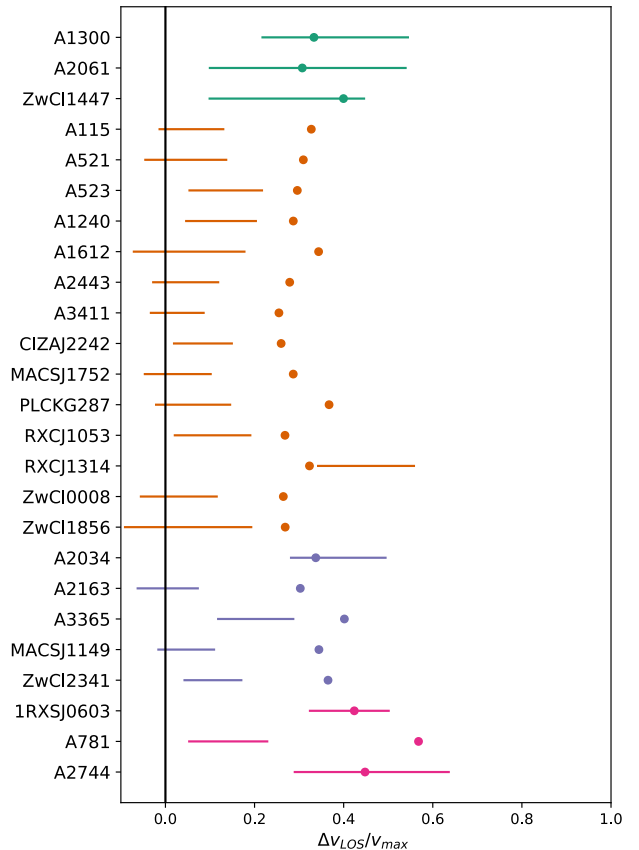
Figure 38. Line of sight velocity differences between merging subclusters associated with radio relics. The clusters are organized by the number of subclusters in the lowest BIC model (see Table 4). Green, orange, purple, and pink refer to systems comprised of one, two, three, and four GMM subclusters, respectively. The bars represent the 95% confidence interval for the ratio of line of sight velocity difference to maximum three dimensional infall velocity. The colored points are the ratio of the global velocity dispersion to the maximum free-fall velocity, for comparison.
