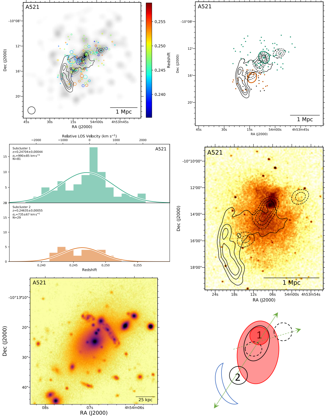
Figure 11. Top left: DS-test over red sequence i-band luminosity distribution with linearly space white contours. The black contours show the 240 MHz GMRT contours (Venturi et al. 2013). Top right: Subcluster membership of spectroscopic cluster members assigned with our GMM analysis. The same GMRT contours (solid) and red sequence luminosity contours (dashed) are depicted. Middle left: Subcluster redshift histograms with colors matching the image at the top right. Middle right: 170 ks Chandra image with the same GMRT radio contours (solid) and red sequence luminosity contours (dashed). A complex merger scenario is evident. Bottom left: 150 kpc cutout of the Subaru/SuprimeCam i-band image centered on the BCG of subcluster 1. The multiple images of the face on spiral are evident. Bottom right: Proposed merger scenario. Dashed black circles correspond to galaxy substructure not identified by the GMM analysis. The dark red region corresponds to the dense ICM core coincident with the BCG.
