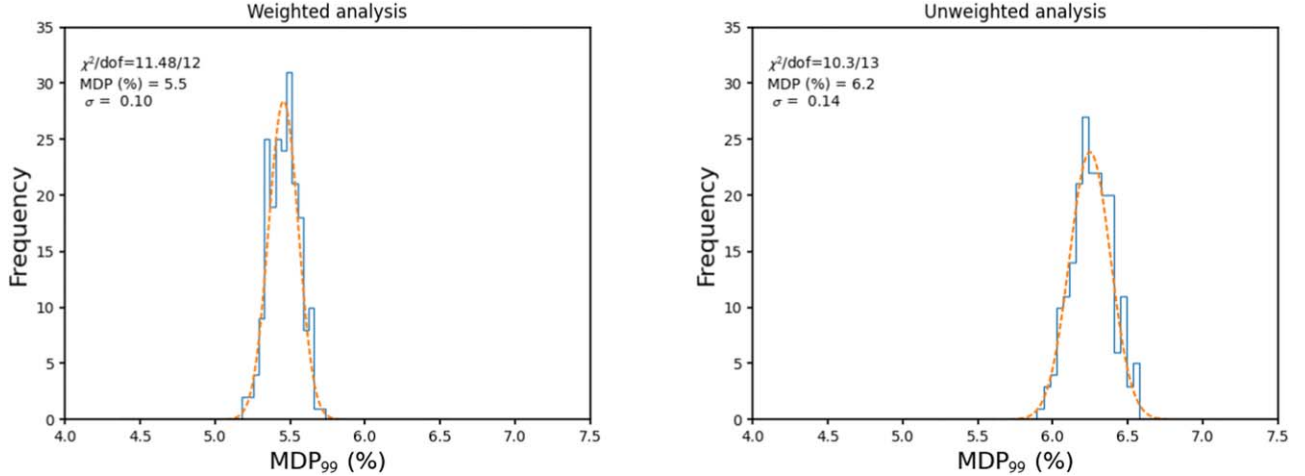
Figure 8. Distribution of MDP 99 values for 200 IXPE simulated observations of a point-like source with energy spectrum described by a power law with number index -2 , a flux 10^{-11} erg cm -2 s -1 in the energy range 2–8 keV, and 10 days of integration time. MDP 99 values are estimated for weighted (left) and unweighted (right) analysis. See text.
