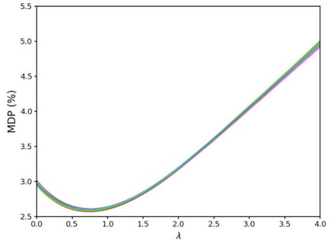
Figure 6. \text{MDP}_{99} values as a function of \lambda for 10 different Monte Carlo simulations. All these distributions have a minimum around \lambda = 0.75 .
