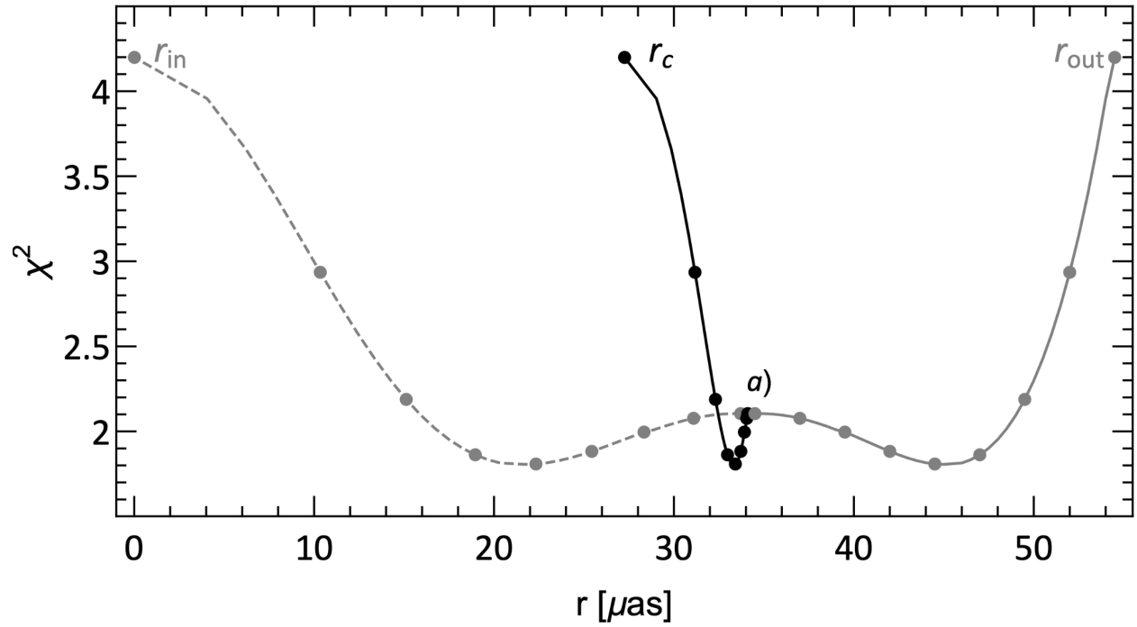
Figure S12 | Evolution of the \chi^2 goodness-of-fit parameter. Reduced \chi^2 is obtained from fitting the jet-subtracted dataset with the thick ring models calculated for outer ring radii, r_{\text{out}} , ranging from 34.5 \mu\text{as} to 54.5 \mu\text{as} . The respective mean, r_c (solid line), and inner, r_{\text{in}} (dashed line), ring radii are also shown. Dots indicate the fits by the subset of the models shown in Figure S13, with the symbol a) indicating the first (top left) model in that figure.
