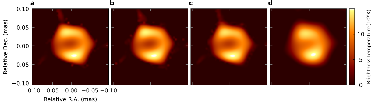
Figure S6| Dependence of the ring-like structure on SMILI regularizers. Images are reconstructed with the hyper parameter (weight) on the total squared variation (TSV) varying from 0 (a) to 10 (b) to 100 (c) to 1000 (d). All other imaging parameters are fixed (total flux = 0.7 Jy, weighted-L1 = 1, TV = 0, MEM = 0, and Gaussian FWHM = 50 \mu as for convolution of the pre-processed image used as prior for wL1, see Supplementary section 3 for details).
