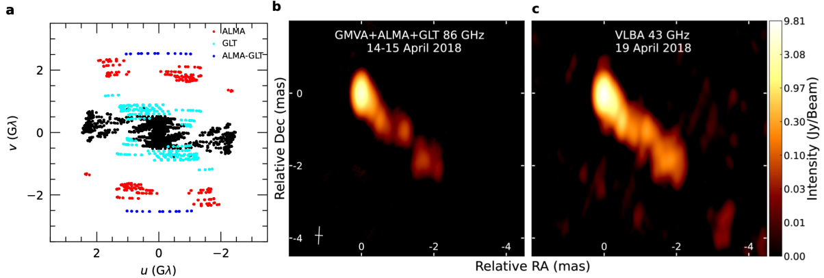
Figure S5 | (u,v) -coverage and CLEAN images of the calibrator 3C273. a , The participation of phased ALMA and GLT greatly improved the (u,v) -coverage to 3C273 (highlighted). b , Total intensity image of 3C 273 obtained from our GMVA+ALMA+GLT observations at 3.5 mm on 14-15 April 2018. c , VLBA image of 3C 273 at 7 mm obtained from observations on 19 April 2018. Both images are restored with the same synthesised beam of FWHM of 0.46 \times 0.20 mas, for the major and minor axis respectively. The beam orientation at a position angle of -3.1^\circ is indicated by the white cross on the bottom left of b .
