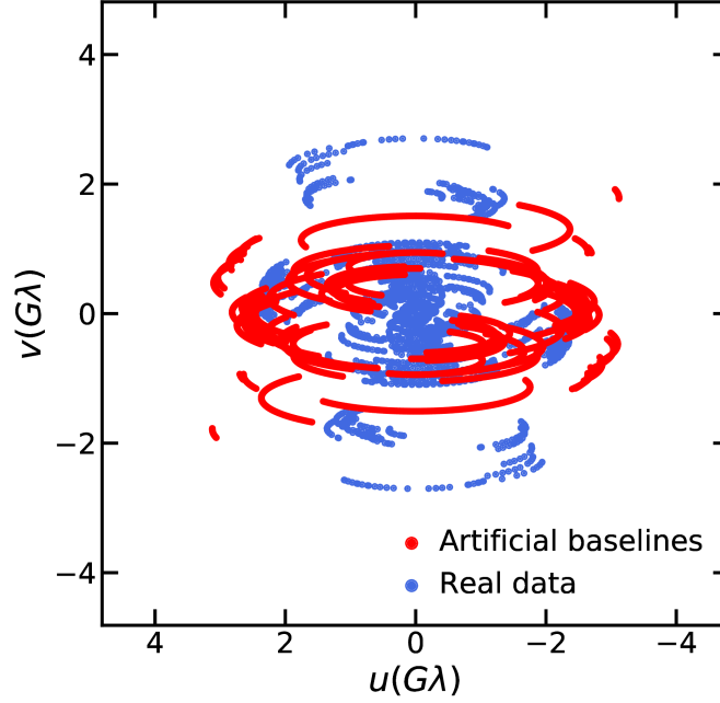
Figure S7 | (u,v) -coverage of the simulated data. Simulated (u,v) -coverage for the 2018 observations of M87 (blue) and for the additional baselines to VLBA MK in Hawaii, USA and KVN Yonsei in South Korea (red), added for the purpose of investigating the effects of (u,v) -coverage on the results.
