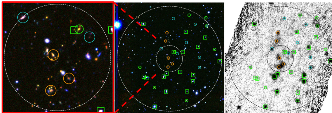
Figure 1. Ks/I colour composite of the central \sim 500 kpc (left) of the field of XDCP0044 (middle) and corresponding Herschel /PACS 100 \mu\text{m} map (right). Dashed circles have radii of 30 arcsec and 2 arcmin centred on the cluster X-ray centre. The five spectroscopic members with FIR emission are shown in orange circles, cyan regions indicate the photometric candidates with FIR emission and green regions correspond to spectroscopic (circles) and visual/photo- z (squares) interlopers.
