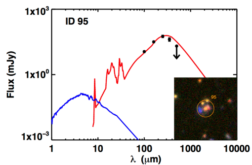
Figure 2. Best-fitting FIR SED (red line) of cluster member ID 95, with Ks/II inset (15 arcsec \times 15 arcsec). Data points are shown in black.
