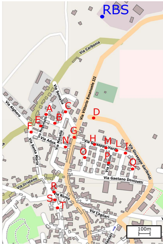
Fig. 10. Geometry of Lunamatrona measurement campaign at 2142.4 MHz. Both the RBS position and the measurement points are shown. The RBS height is 20 m and the RBS pointing direction is 190^\circ .
