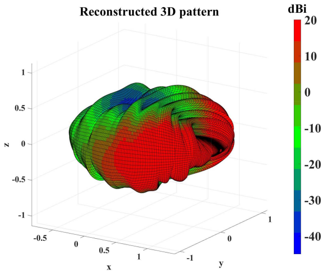
Fig. 5. Reconstructed tridimensional pattern for the Kathrein 730376 antenna using the explained algorithm.
