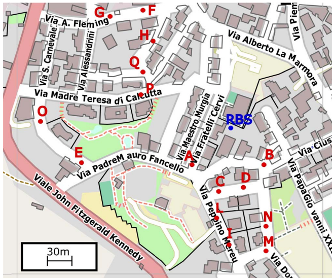
Fig. 8. Geometry of Dorgali measurement campaign at 944.2 MHz. Both the RBS position and the measurement points are shown. The RBS height is 20 m and its pointing direction is 300^\circ .
