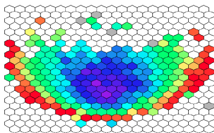
Figure 55: A typical ELVES candidate event as seen in the FD.
