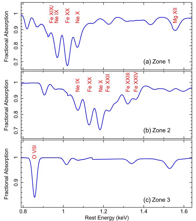
Figure 10. A graphical representation of the three XSTAR absorber zones (see Table 4), showing the fraction of the continuum absorbed by each zone in the region around 1 keV. Zone 1 (upper panel) corresponds to the lowest velocity (0.06 c ), lower ionization component in OBS. E, which mainly produces the 1 keV absorption trough seen in this observation. Zone 2 (middle panel) is a faster zone, and the blend of lines is responsible for the broad absorption trough observed near 1.2 keV. Most of the contribution to zones 1 and 2 arises from the L-shell lines of iron and K-shell Ne. Zone 3 (lower panel) is the highest ionization and fastest zone present in OBS. CD, which makes only a small contribution to the soft band, as it is mainly responsible for the blueshifted absorption near 0.8 keV, which is due to O VIII Ly \alpha .
