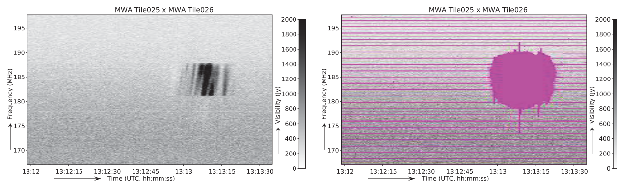
Figure 7. DTV RFI briefly visible in an EoR high-band observation. The plots show the Stokes I amplitudes for a single correlation. The right plot shows the result of RFI detection and invalid channels marked in purple.
