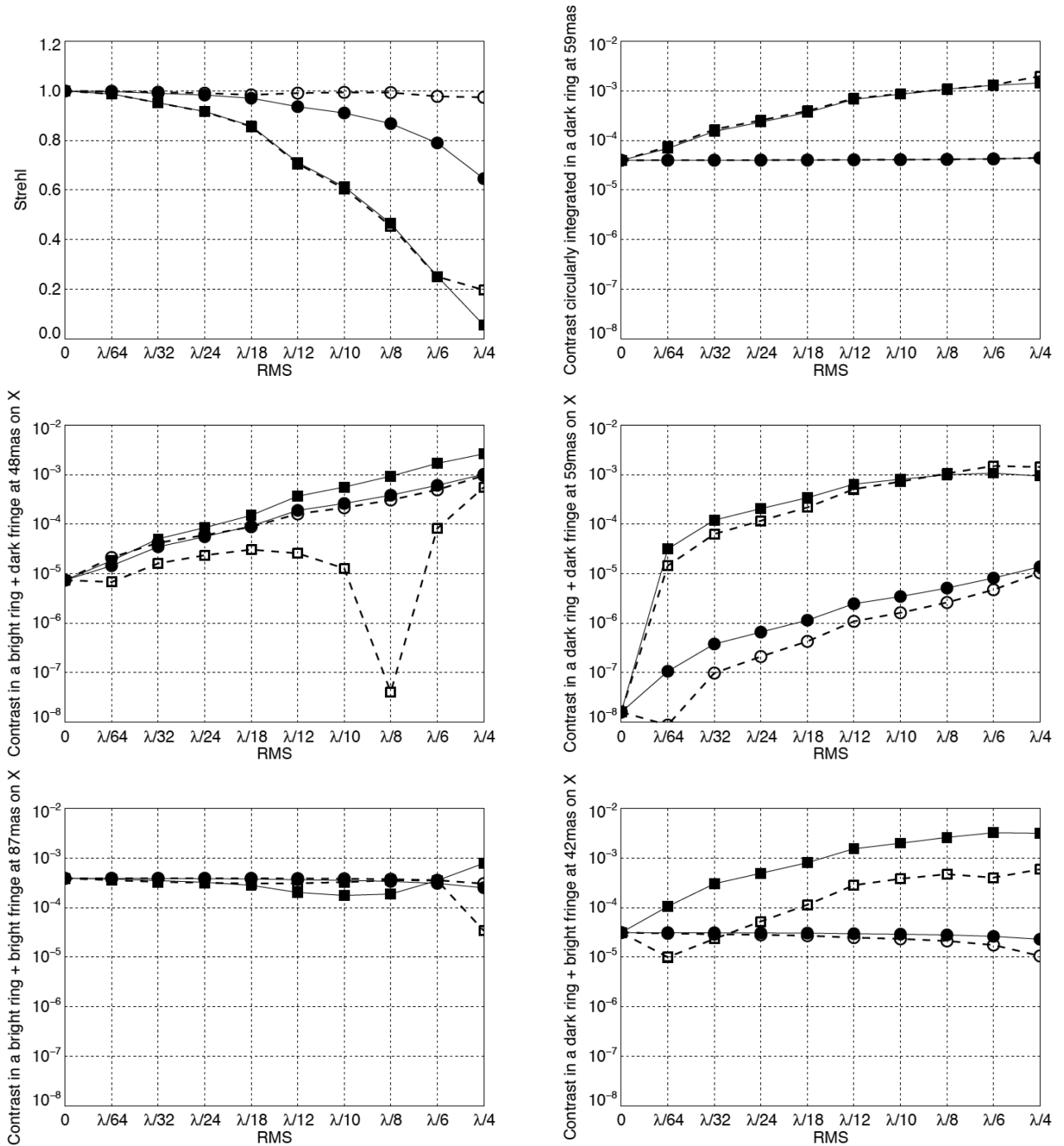
Figure 6. Merit functions for the PSF: interferometric Strehl (top left), contrast circularly integrated in a dark ring at 59 mas (top right), contrast on X in a bright ring and a dark fringe at 48 mas (middle left), contrast on the X axis in a dark ring and a dark fringe at 59 mas (middle right), contrast on X in a bright ring and a bright fringe at 87 mas (bottom left), contrast on X in a dark ring and a bright fringe at 42 mas (bottom right). AO wavefront errors (square symbol) or piston errors (circular symbol) for different RMS values. Short exposure (empty symbol, dashed line) and long exposure (filled symbol, solid line).
