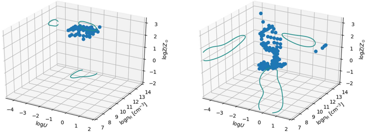
Figure 12. Parameter space n_H , U , Z . Left: data points in 3D space are elements in the grid of the parameter space selected for not being different from \chi^2_{\min} by more than \delta\chi^2 \approx 1 , computed from the emission-line ratios measured for the BC and referring to the median values in Table 5. Right: same as the left panel, but for the BLUE component, also including the condition that the data points are in agreement with the three diagnostic ratios within the SIQR of the median estimate from Table 5. The individual contour line was smoothed with a Gaussian kernel.
