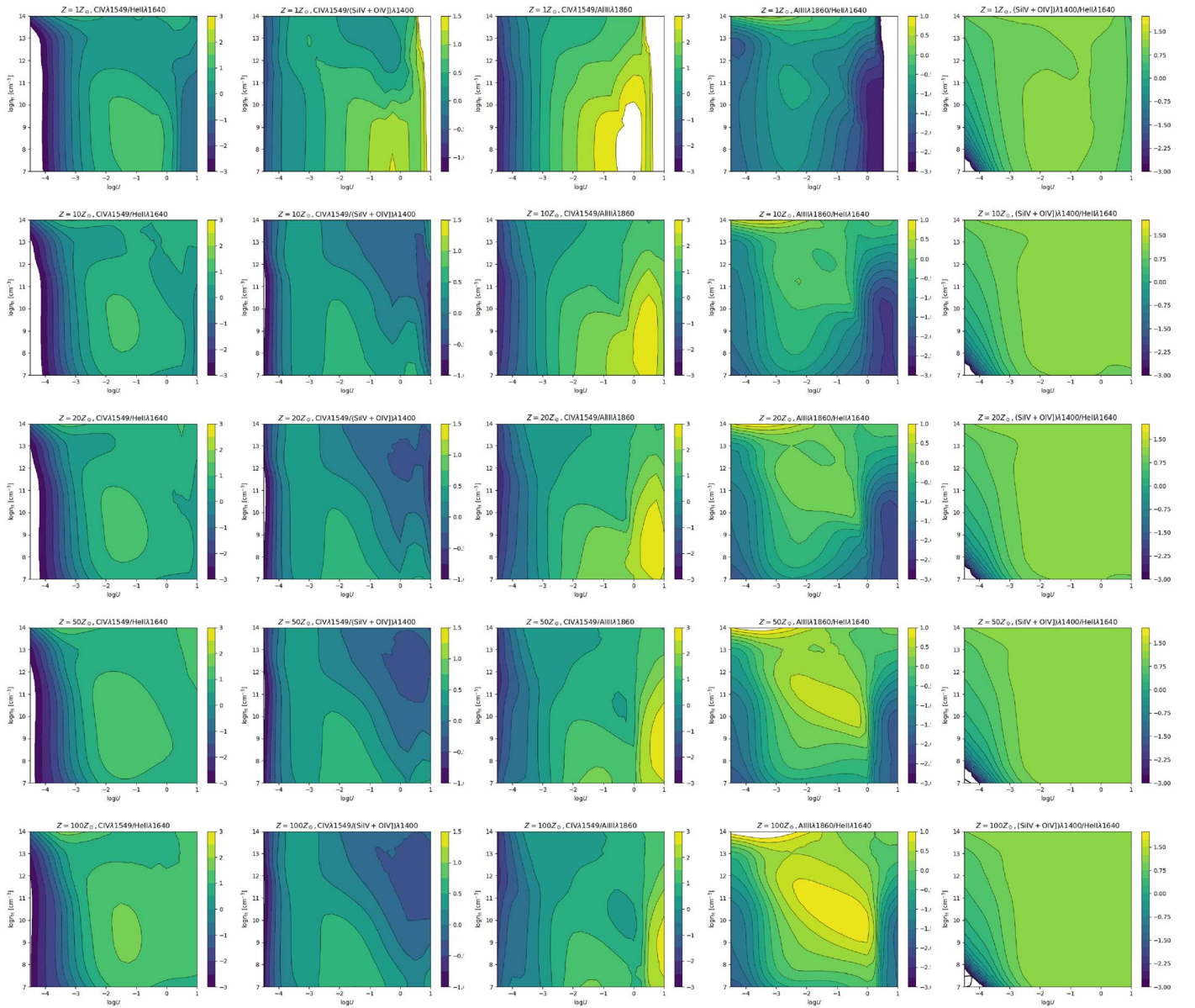
Figure 18. Isophotal contour in the \log U – \log n_H for line intensity ratios (from left to right) C IV/He II, C IV/(Si IV + O IV), C IV/Al III, Al III/He II \lambda 1640 , (Si IV + O IV)/He II \lambda 1640 as a function of metallicity (from top to bottom: Z = 1, 10, 20, 50, 100 Z_\odot ), for column density N_e = 10^{23} \text{ cm}^{-2} .
