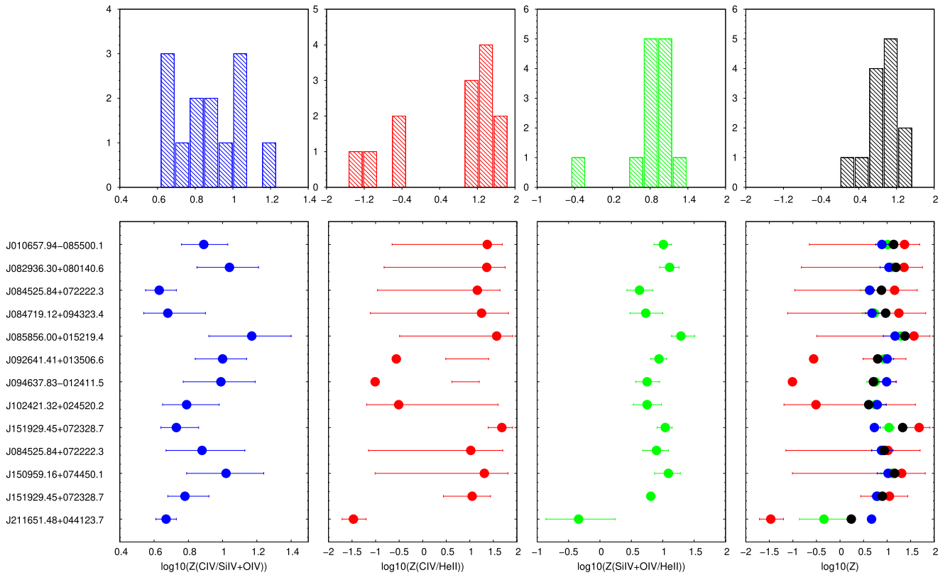
Figure 11. Top panels: distribution of metallicity measurements for blue component obtained from ratios C IV/Si IV + O IV (blue), C IV/He II λ1640 (red), and Si IV + O IV/He II λ1640 (green), and the mean metallicity obtained from all ratios (black). Bottom panels: results and associated uncertainties for individual sources with the same color-coding as histograms. The last panel contains all metallicity measurements and the mean of them for each object.
