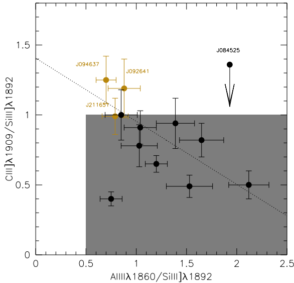
Figure 6. Relation between intensity ratios Al III \lambda 1860 /Si III] \lambda 1892 and C III] \lambda 1909 /Si III] \lambda 1892 . The gray area corresponds to the parameter space occupied by the xA sources. Borderline sources are in orange color.
