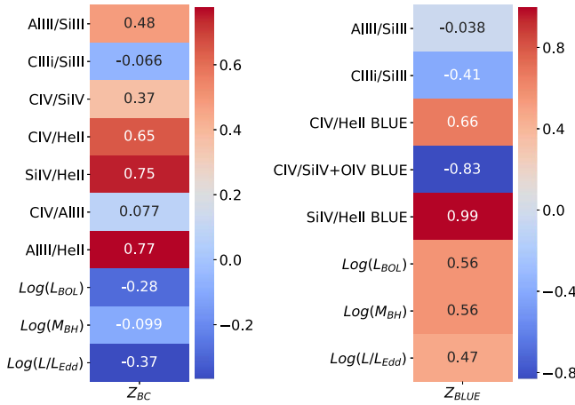
Figure 13. Left panel: correlation matrix between Z computed for the BC and BC diagnostic ratios assuming fixed n_H and U along with log of bolometric luminosity, log of black hole mass, and log of Eddington ratio. Right panel: same as the left panel, but for the BLUE component. The numbers in each square show the Spearman rank correlation coefficient. The color hue is proportional to the correlation, from dark blue (strong negative correlation) to red (strong positive correlation).
